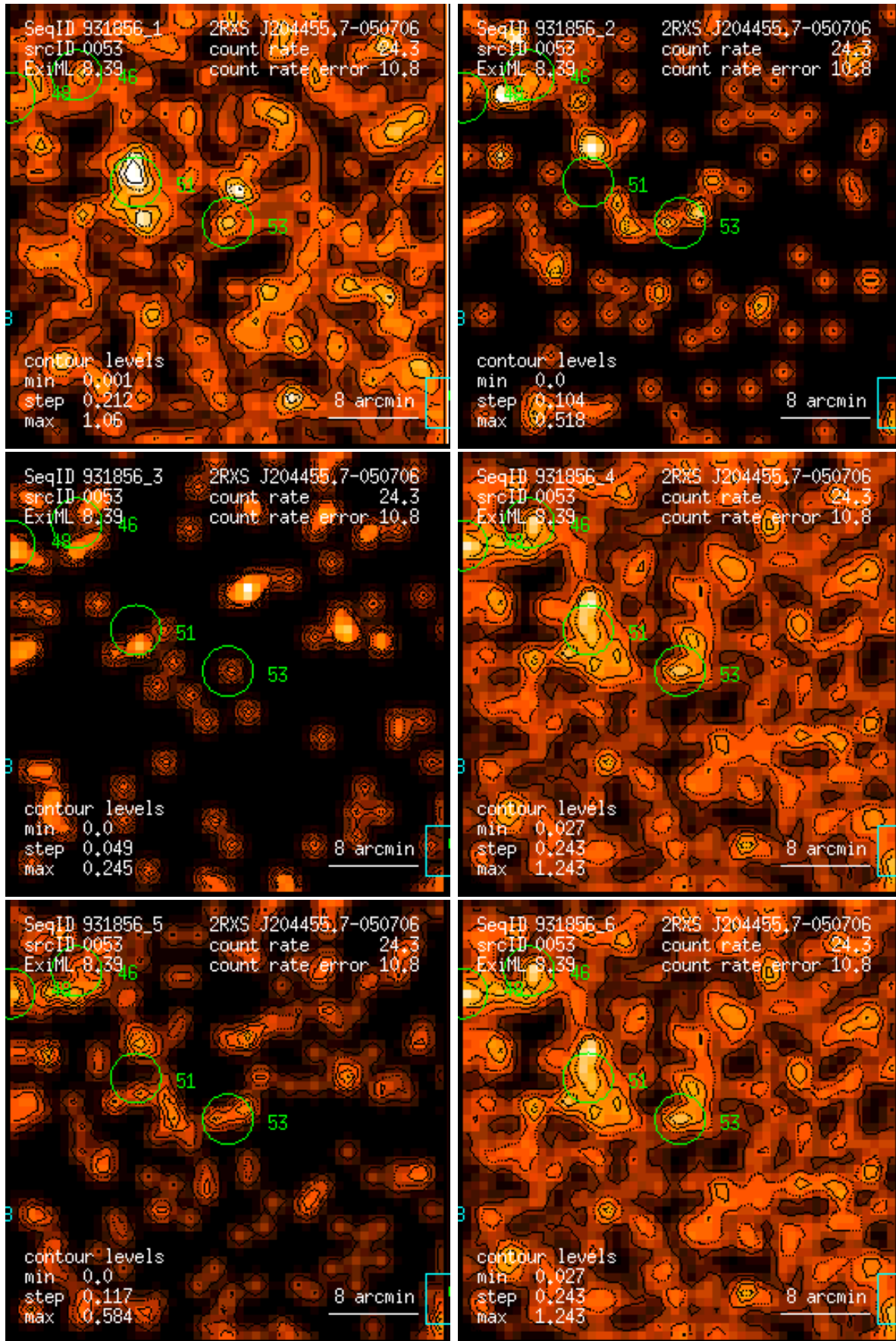
Figure 53: RASS 931856: detection 0053: band rate images, Gaussian filter: (1) PSPC channels 11 – 41, (2) 52 – 90, (3) 91 – 201, (4) 11 – 235, (5) 52 – 201, (6) 11 – 201. Broad band rates in counts/ks. Band rate contour levels in counts/ks/arcmin 2 .
