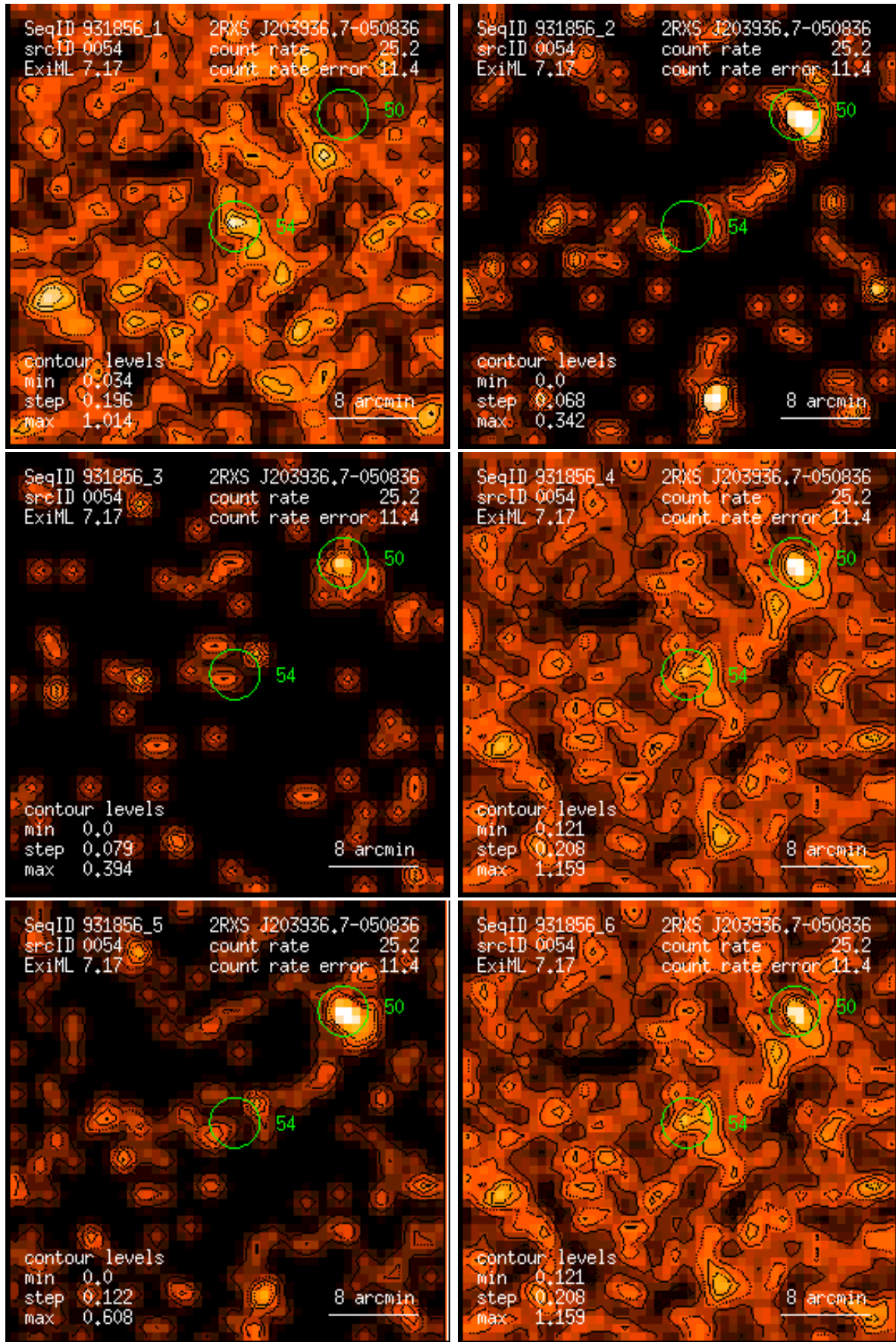
Figure 54: RASS 931856: detection 0054: band rate images, Gaussian filter: (1) PSPC channels 11 – 41, (2) 52 – 90, (3) 91 – 201, (4) 11 – 235, (5) 52 – 201, (6) 11 – 201. Broad band rates in counts/ks. Band rate contour levels in counts/ks/arcmin 2 .
