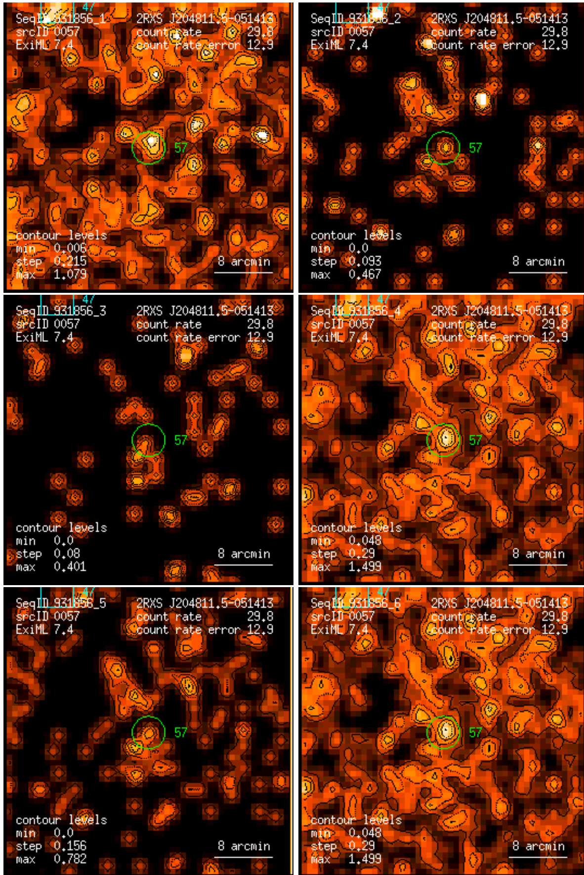
Figure 57: RASS 931856: detection 0057: band rate images, Gaussian filter: (1) PSPC channels 11 – 41, (2) 52 – 90, (3) 91 – 201, (4) 11 – 235, (5) 52 – 201, (6) 11 – 201. Broad band rates in counts/ks. Band rate contour levels in counts/ks/arcmin 2 .
