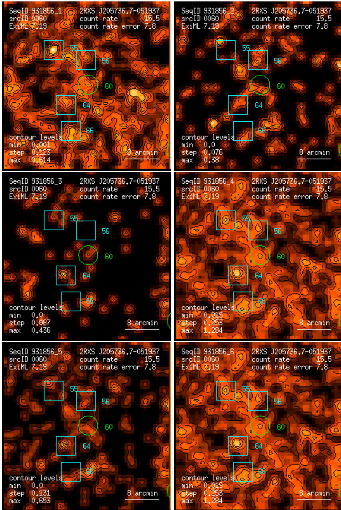
Figure 60: RASS 931856: detection 0060: band rate images, Gaussian filter: (1) PSPC channels 11 – 41, (2) 52 – 90, (3) 91 – 201, (4) 11 – 235, (5) 52 – 201, (6) 11 – 201. Broad band rates in counts/ks. Band rate contour levels in counts/ks/arcmin 2 .
