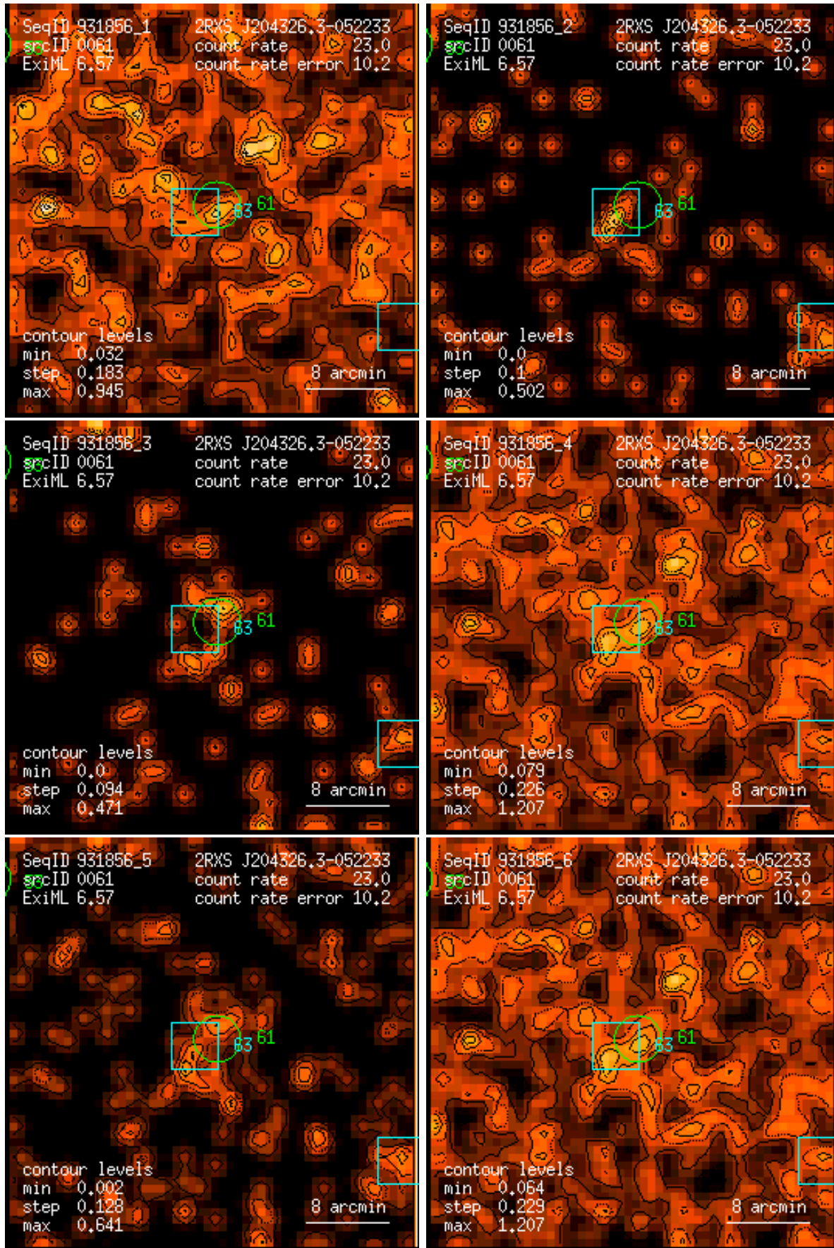
Figure 61: RASS 931856: detection 0061: band rate images, Gaussian filter: (1) PSPC channels 11 – 41, (2) 52 – 90, (3) 91 – 201, (4) 11 – 235, (5) 52 – 201, (6) 11 – 201. Broad band rates in counts/ks. Band rate contour levels in counts/ks/arcmin 2 .
