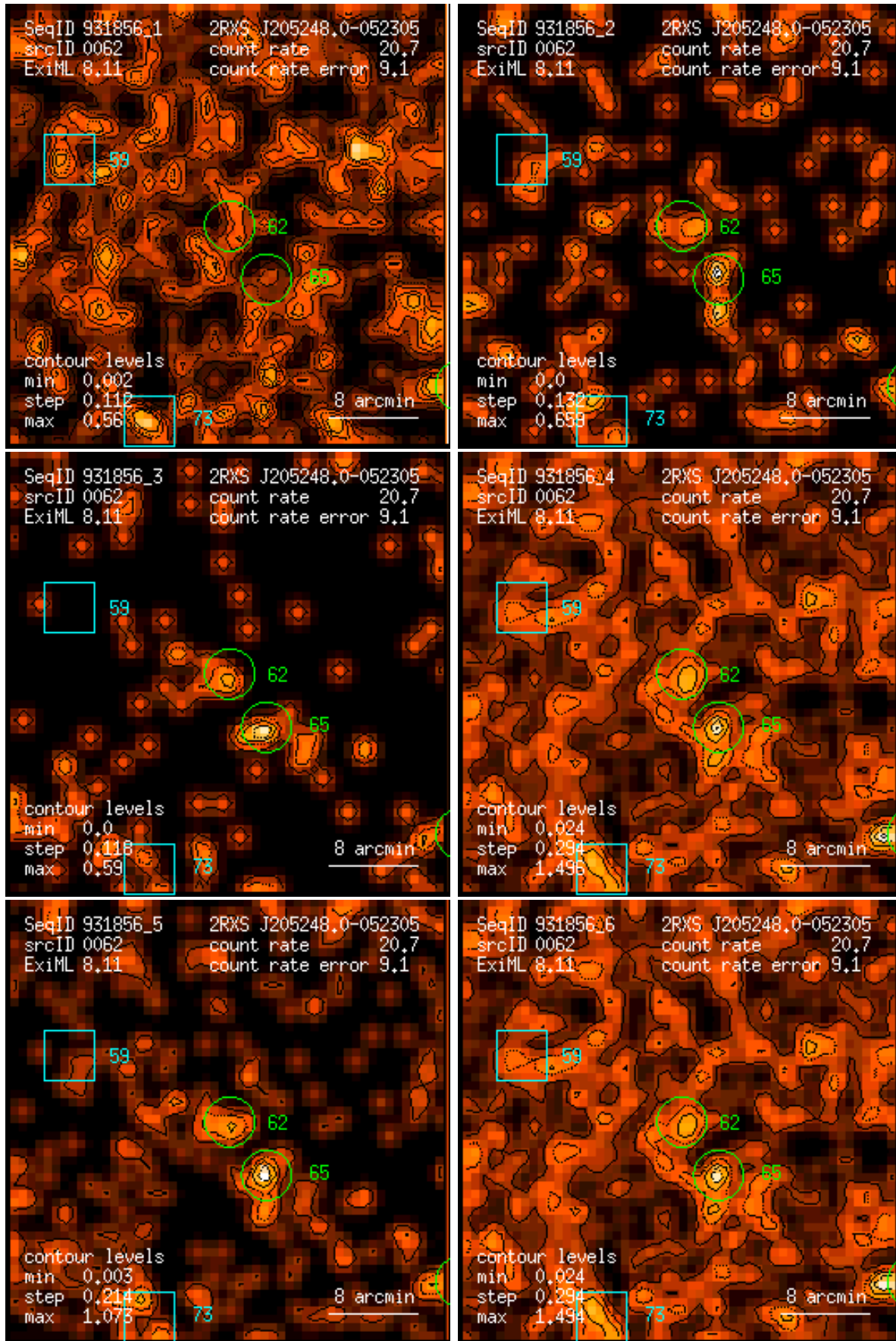
Figure 62: RASS 931856: detection 0062: band rate images, Gaussian filter: (1) PSPC channels 11 – 41, (2) 52 – 90, (3) 91 – 201, (4) 11 – 235, (5) 52 – 201, (6) 11 – 201. Broad band rates in counts/ks. Band rate contour levels in counts/ks/arcmin 2 .
