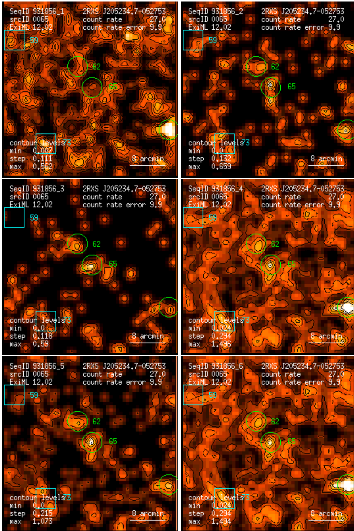
Figure 65: RASS 931856: detection 0065: band rate images, Gaussian filter: (1) PSPC channels 11 – 41, (2) 52 – 90, (3) 91 – 201, (4) 11 – 235, (5) 52 – 201, (6) 11 – 201. Broad band rates in counts/ks. Band rate contour levels in counts/ks/arcmin 2 .
