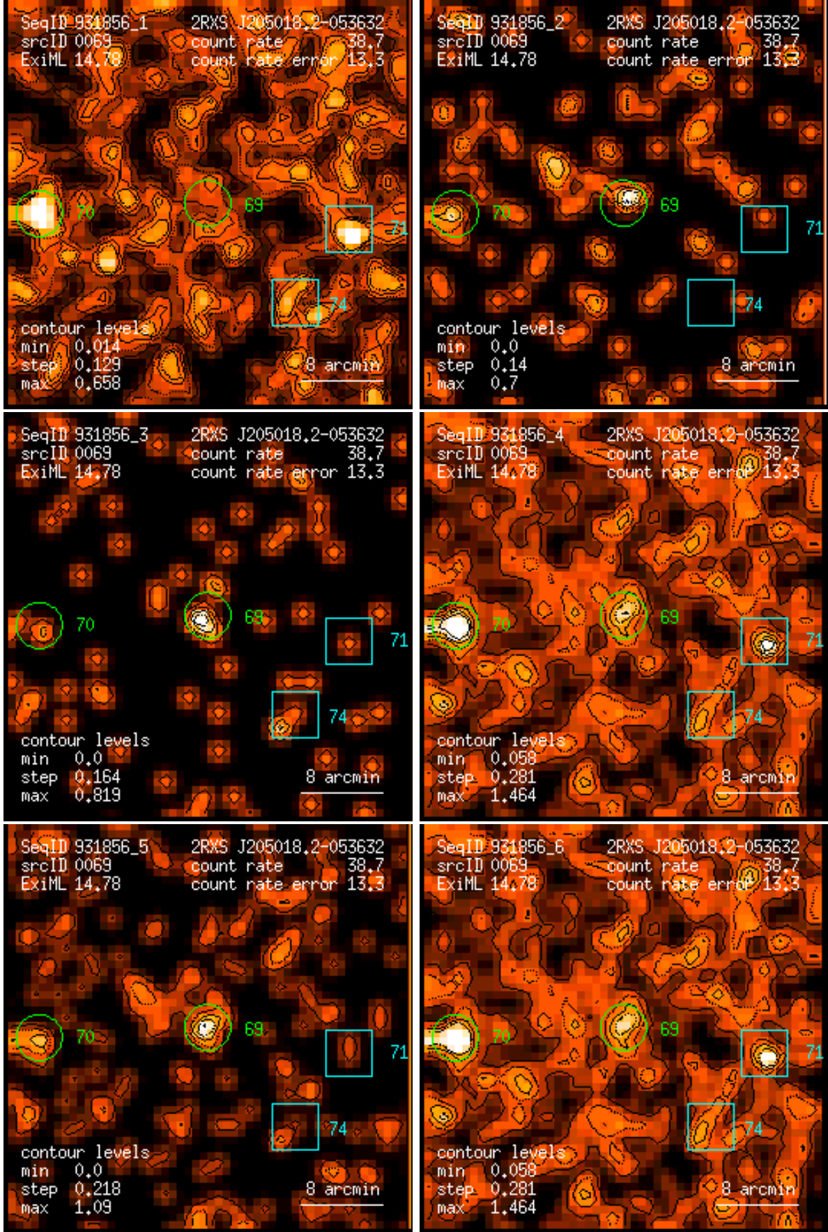
Figure 69: RASS 931856: detection 0069: band rate images, Gaussian filter: (1) PSPC channels 11 – 41, (2) 52 – 90, (3) 91 – 201, (4) 11 – 235, (5) 52 – 201, (6) 11 – 201. Broad band rates in counts/ks. Band rate contour levels in counts/ks/arcmin 2 .
