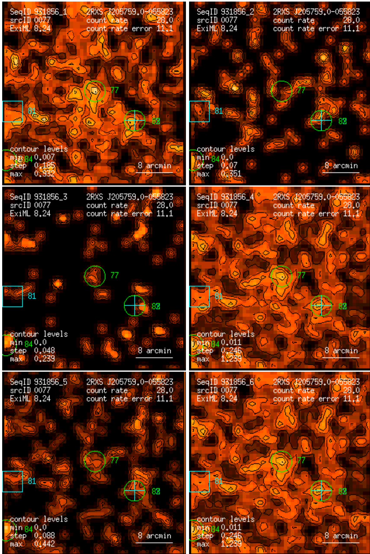
Figure 77: RASS 931856: detection 0077: band rate images, Gaussian filter: (1) PSPC channels 11 – 41, (2) 52 – 90, (3) 91 – 201, (4) 11 – 235, (5) 52 – 201, (6) 11 – 201. Broad band rates in counts/ks. Band rate contour levels in counts/ks/arcmin 2 .
