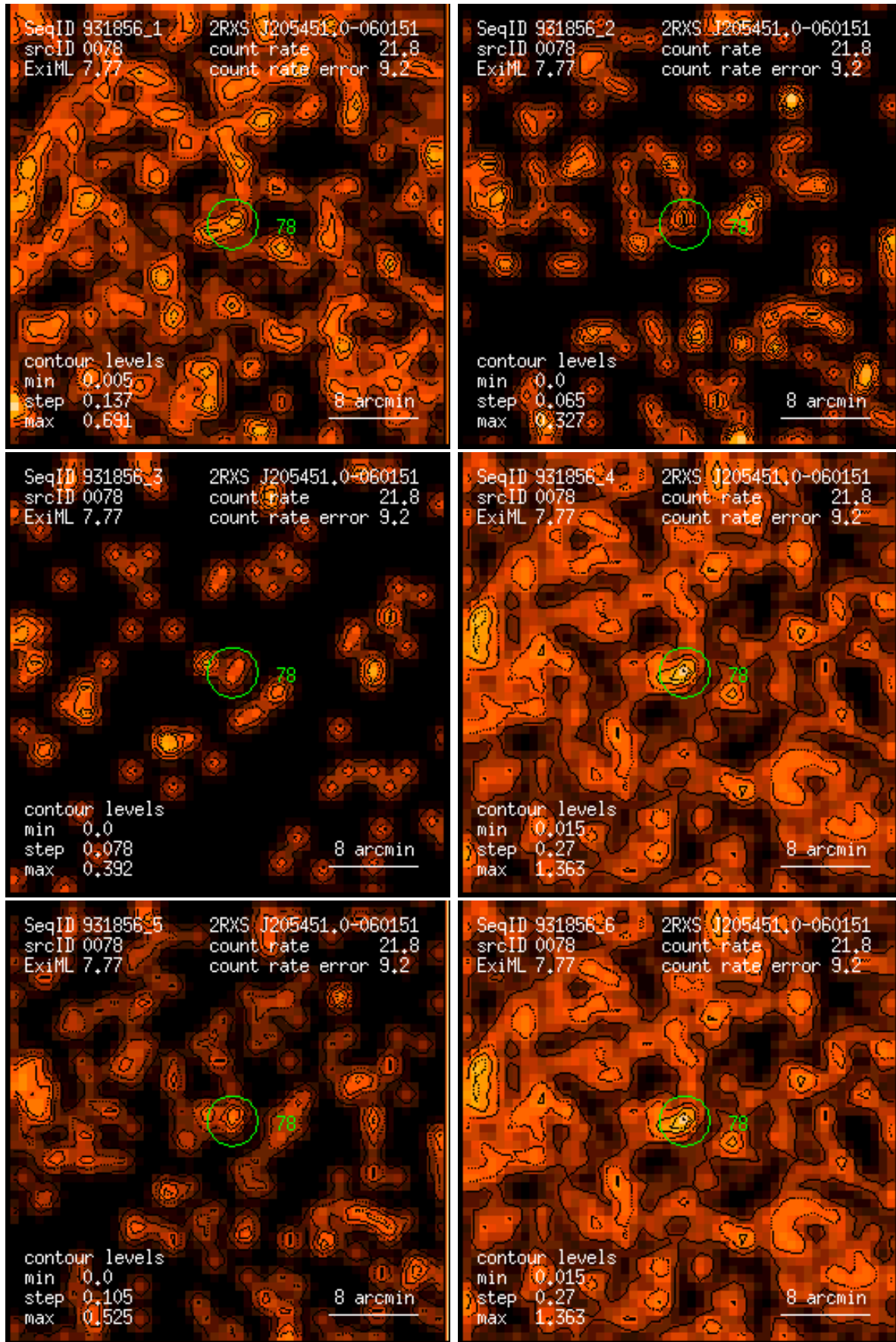
Figure 78: RASS 931856: detection 0078: band rate images, Gaussian filter: (1) PSPC channels 11 – 41, (2) 52 – 90, (3) 91 – 201, (4) 11 – 235, (5) 52 – 201, (6) 11 – 201. Broad band rates in counts/ks. Band rate contour levels in counts/ks/arcmin 2 .
