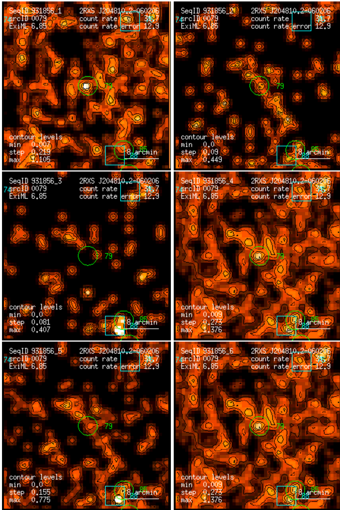
Figure 79: RASS 931856: detection 0079: band rate images, Gaussian filter: (1) PSPC channels 11 – 41, (2) 52 – 90, (3) 91 – 201, (4) 11 – 235, (5) 52 – 201, (6) 11 – 201. Broad band rates in counts/ks. Band rate contour levels in counts/ks/arcmin 2 .
