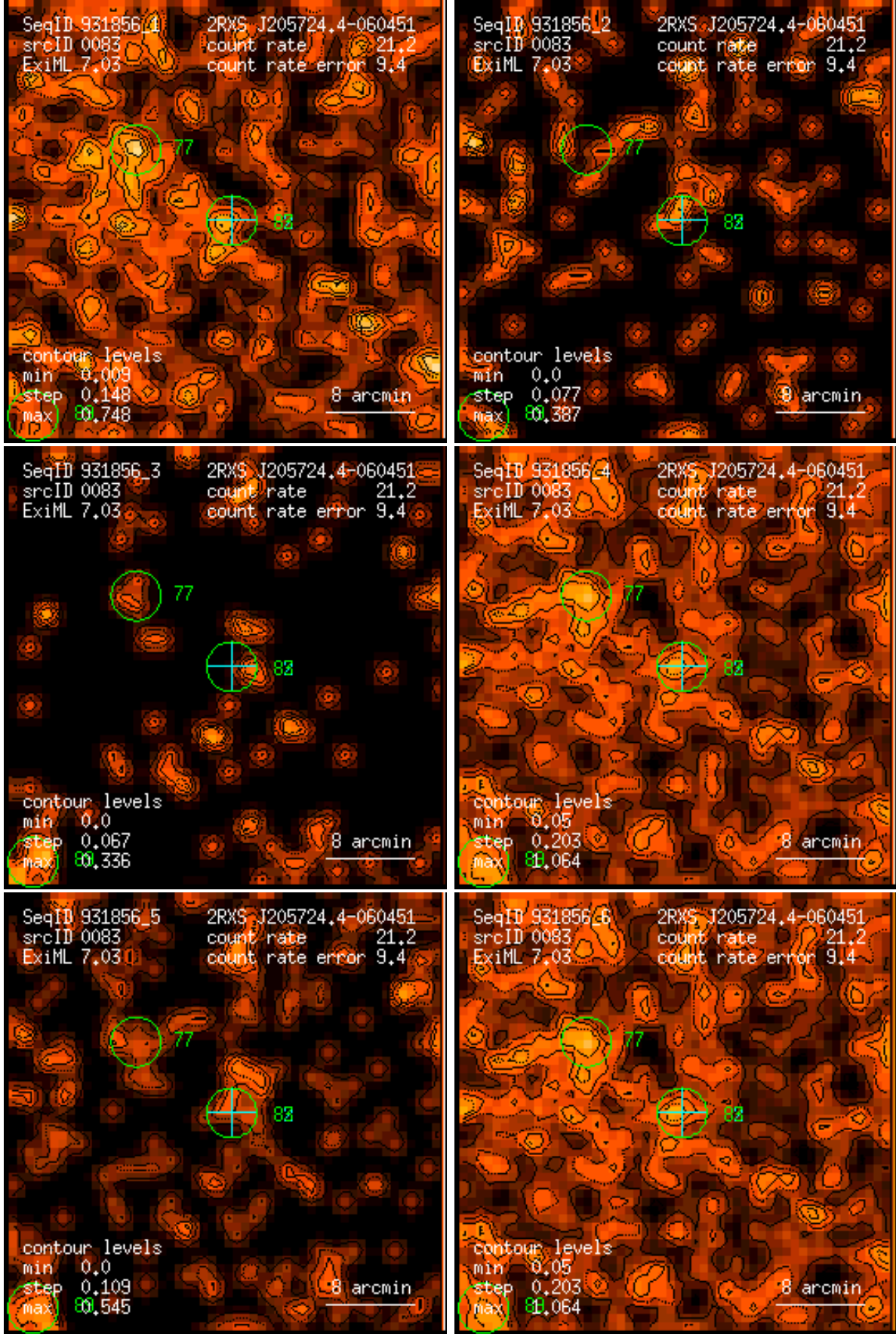
Figure 83: RASS 931856: detection 0083: band rate images, Gaussian filter: (1) PSPC channels 11 – 41, (2) 52 – 90, (3) 91 – 201, (4) 11 – 235, (5) 52 – 201, (6) 11 – 201. Broad band rates in counts/ks. Band rate contour levels in counts/ks/arcmin 2 .
