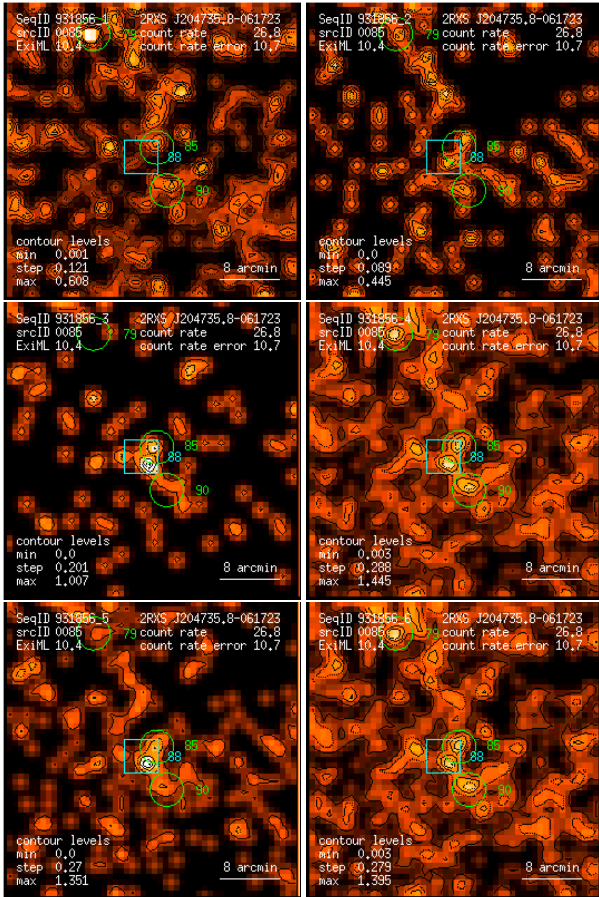
Figure 85: RASS 931856: detection 0085: band rate images, Gaussian filter: (1) PSPC channels 11 – 41, (2) 52 – 90, (3) 91 – 201, (4) 11 – 235, (5) 52 – 201, (6) 11 – 201. Broad band rates in counts/ks. Band rate contour levels in counts/ks/arcmin 2 .
