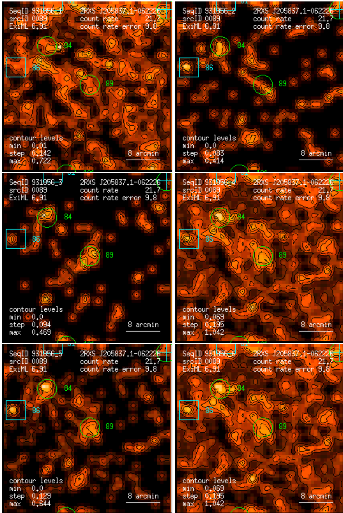
Figure 89: RASS 931856: detection 0089: band rate images, Gaussian filter: (1) PSPC channels 11 – 41, (2) 52 – 90, (3) 91 – 201, (4) 11 – 235, (5) 52 – 201, (6) 11 – 201. Broad band rates in counts/ks. Band rate contour levels in counts/ks/arcmin 2 .
