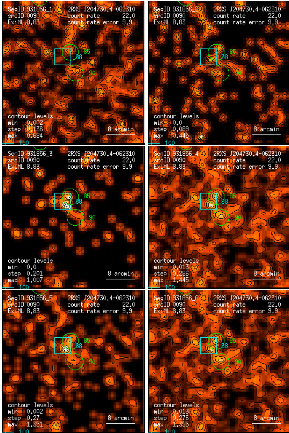
Figure 90: RASS 931856: detection 0090: band rate images, Gaussian filter: (1) PSPC channels 11 – 41, (2) 52 – 90, (3) 91 – 201, (4) 11 – 235, (5) 52 – 201, (6) 11 – 201. Broad band rates in counts/ks. Band rate contour levels in counts/ks/arcmin 2 .
