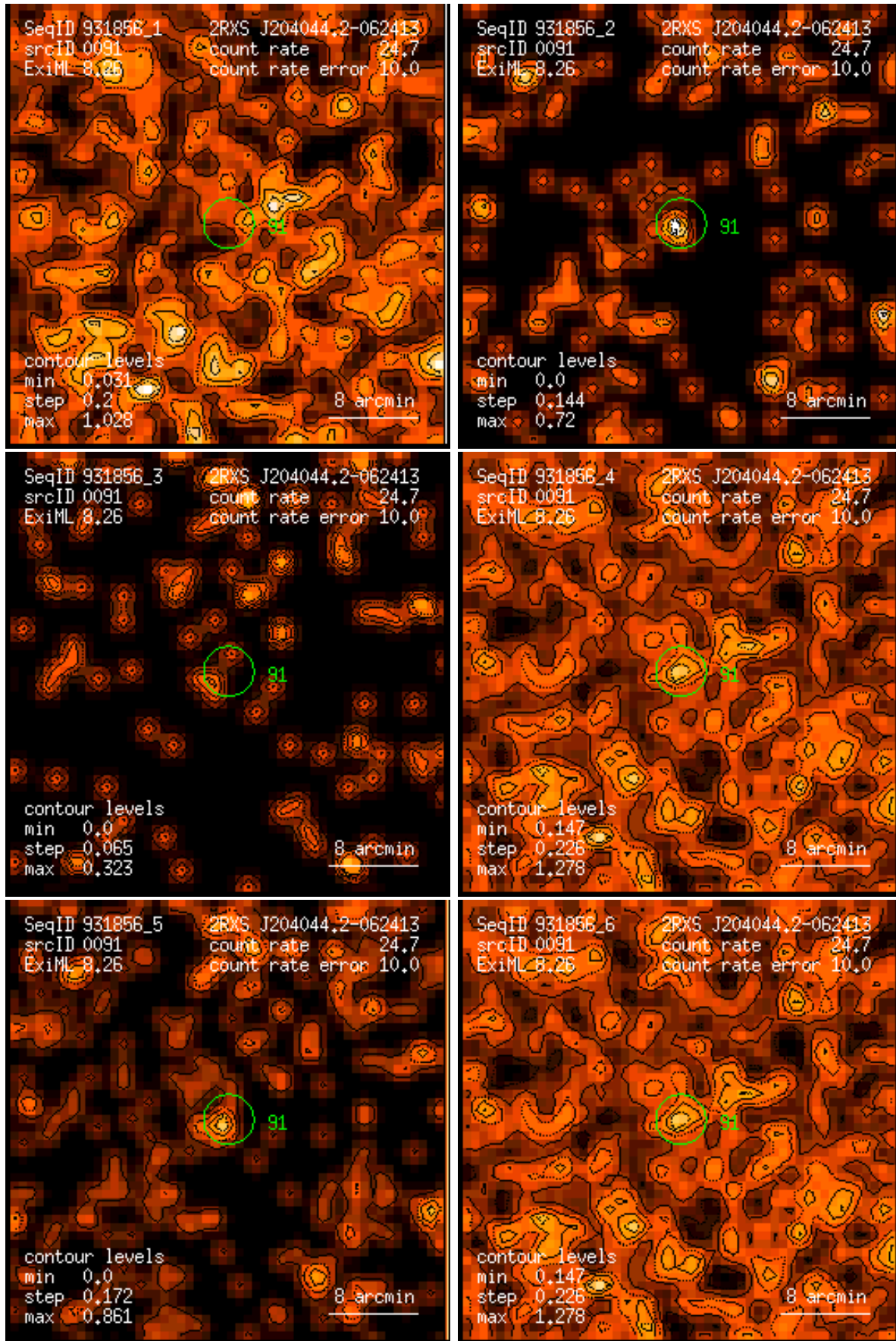
Figure 91: RASS 931856: detection 0091: band rate images, Gaussian filter: (1) PSPC channels 11 – 41, (2) 52 – 90, (3) 91 – 201, (4) 11 – 235, (5) 52 – 201, (6) 11 – 201. Broad band rates in counts/ks. Band rate contour levels in counts/ks/arcmin 2 .
