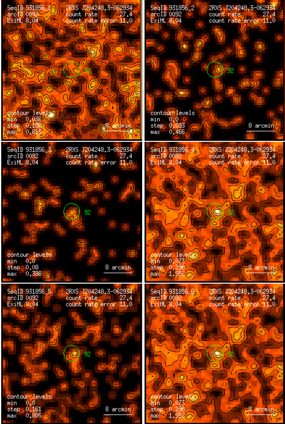
Figure 92: RASS 931856: detection 0092: band rate images, Gaussian filter: (1) PSPC channels 11 – 41, (2) 52 – 90, (3) 91 – 201, (4) 11 – 235, (5) 52 – 201, (6) 11 – 201. Broad band rates in counts/ks. Band rate contour levels in counts/ks/arcmin 2 .
