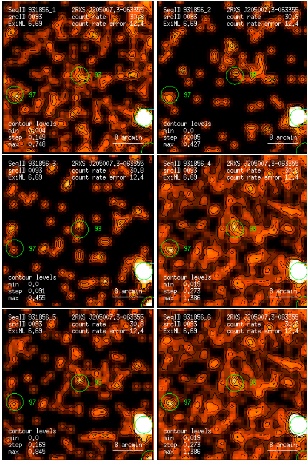
Figure 93: RASS 931856: detection 0093: band rate images, Gaussian filter: (1) PSPC channels 11 – 41, (2) 52 – 90, (3) 91 – 201, (4) 11 – 235, (5) 52 – 201, (6) 11 – 201. Broad band rates in counts/ks. Band rate contour levels in counts/ks/arcmin 2 .
