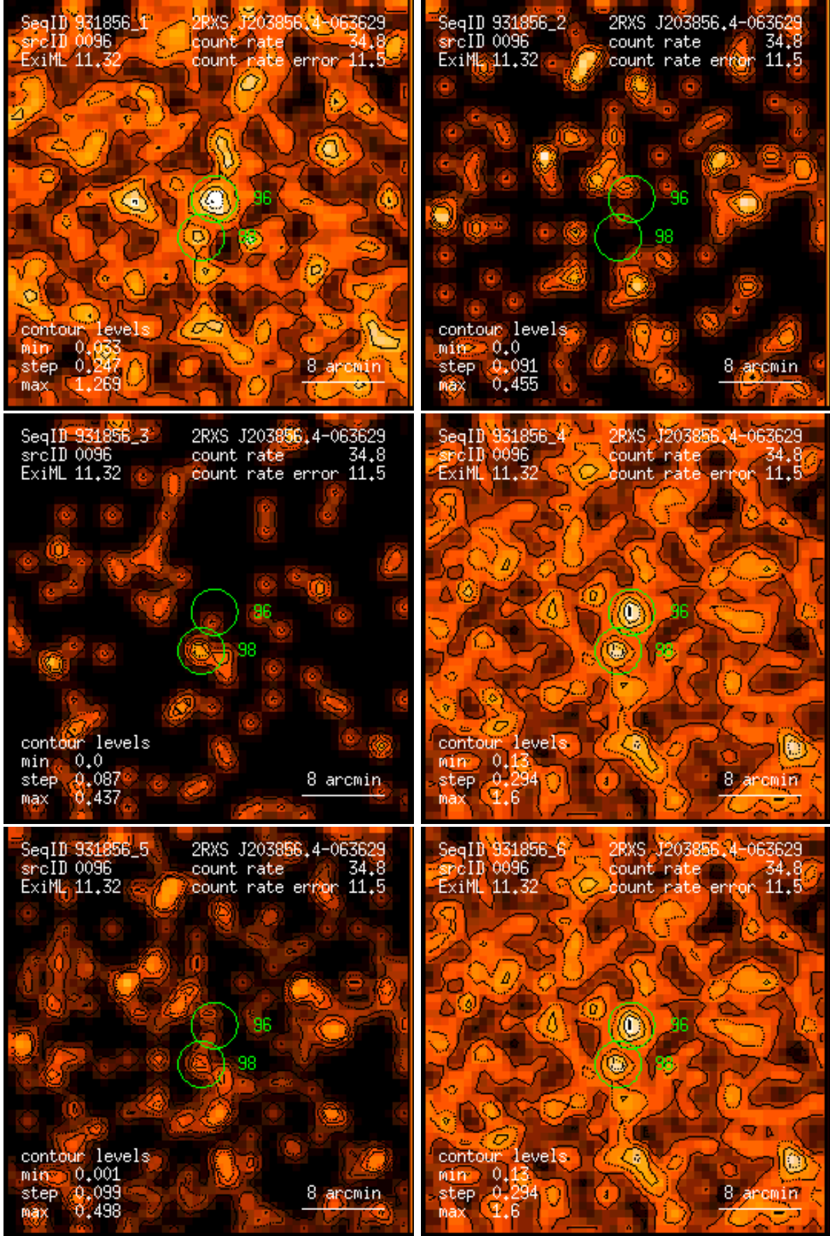
Figure 96: RASS 931856: detection 0096: band rate images, Gaussian filter: (1) PSPC channels 11 – 41, (2) 52 – 90, (3) 91 – 201, (4) 11 – 235, (5) 52 – 201, (6) 11 – 201. Broad band rates in counts/ks. Band rate contour levels in counts/ks/arcmin 2 .
