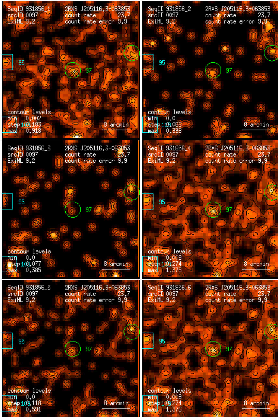
Figure 97: RASS 931856: detection 0097: band rate images, Gaussian filter: (1) PSPC channels 11 – 41, (2) 52 – 90, (3) 91 – 201, (4) 11 – 235, (5) 52 – 201, (6) 11 – 201. Broad band rates in counts/ks. Band rate contour levels in counts/ks/arcmin 2 .
