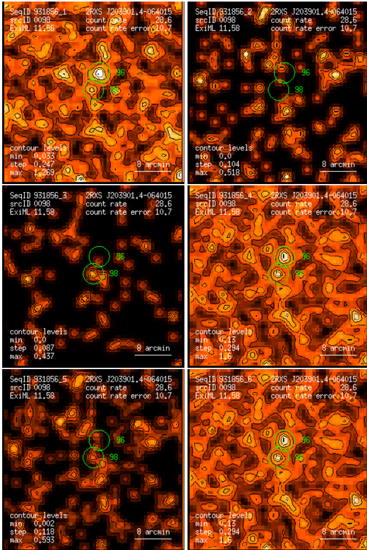
Figure 98: RASS 931856: detection 0098: band rate images, Gaussian filter: (1) PSPC channels 11 – 41, (2) 52 – 90, (3) 91 – 201, (4) 11 – 235, (5) 52 – 201, (6) 11 – 201. Broad band rates in counts/ks. Band rate contour levels in counts/ks/arcmin 2 .
