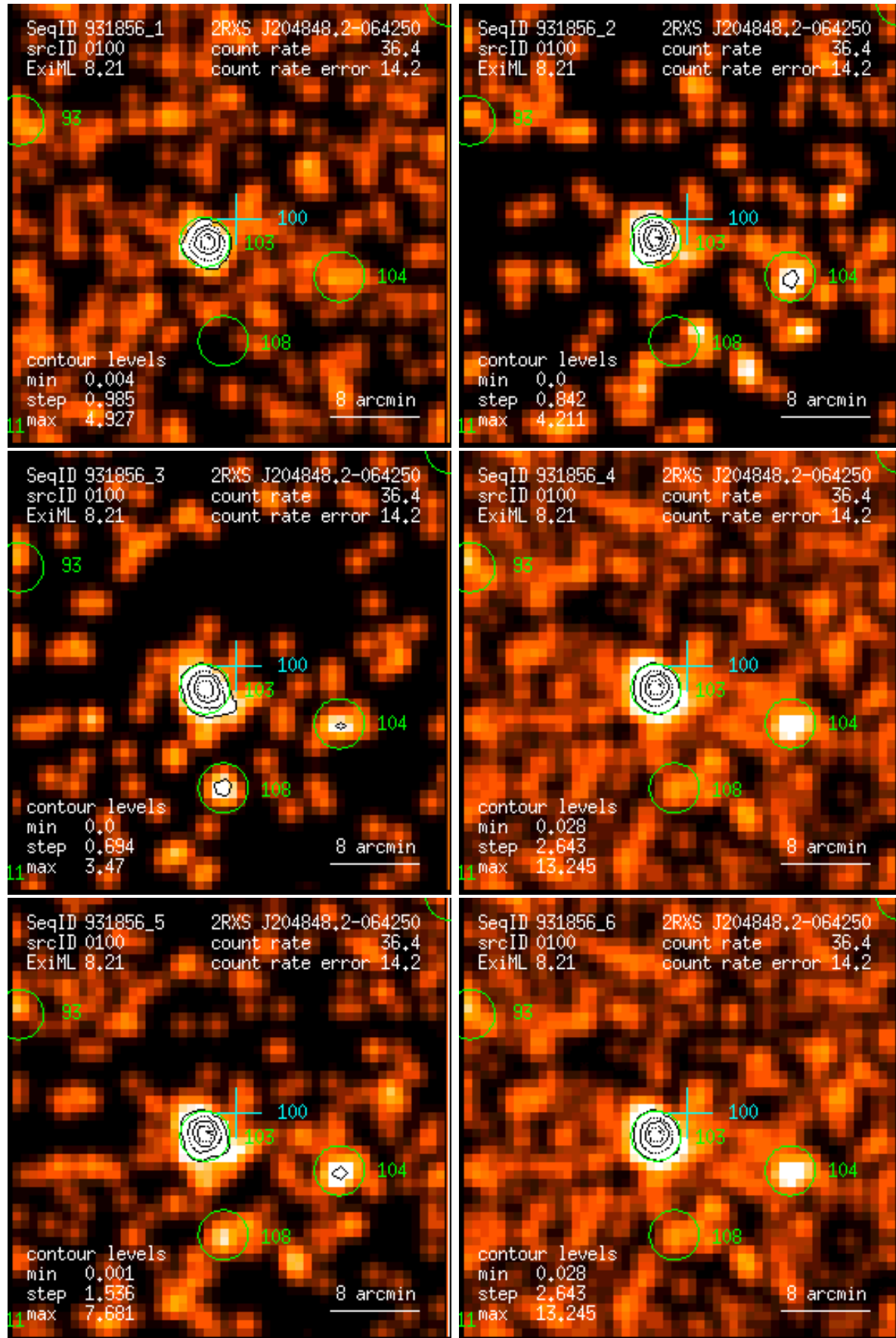
Figure 100: RASS 931856: detection 0100: band rate images, Gaussian filter: (1) PSPC channels 11 – 41, (2) 52 – 90, (3) 91 – 201, (4) 11 – 235, (5) 52 – 201, (6) 11 – 201. Broad band rates in counts/ks. Band rate contour levels in counts/ks/arcmin 2 .
