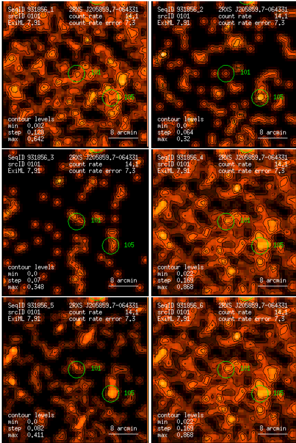
Figure 101: RASS 931856: detection 0101: band rate images, Gaussian filter: (1) PSPC channels 11 – 41, (2) 52 – 90, (3) 91 – 201, (4) 11 – 235, (5) 52 – 201, (6) 11 – 201. Broad band rates in counts/ks. Band rate contour levels in counts/ks/arcmin 2 .
