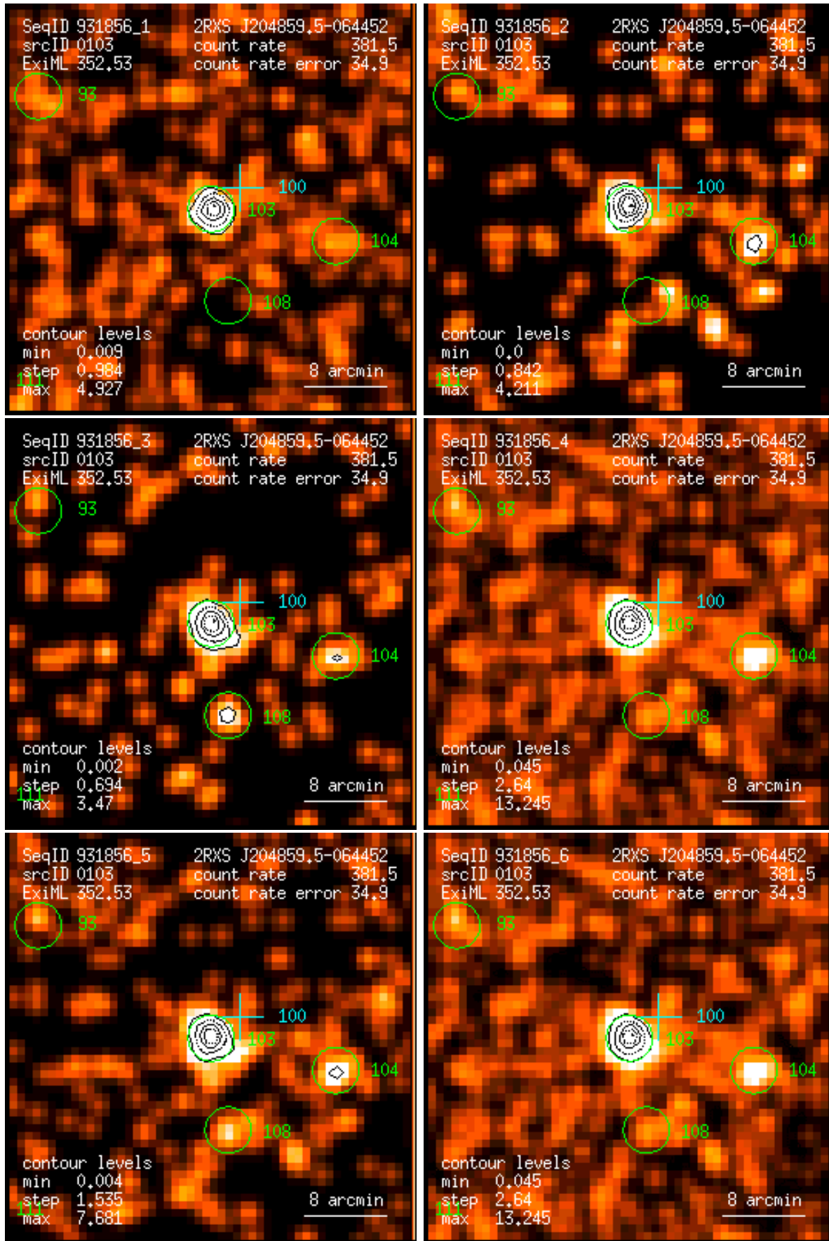
Figure 103: RASS 931856: detection 0103: band rate images, Gaussian filter: (1) PSPC channels 11 – 41, (2) 52 – 90, (3) 91 – 201, (4) 11 – 235, (5) 52 – 201, (6) 11 – 201. Broad band rates in counts/ks. Band rate contour levels in counts/ks/arcmin 2 .
