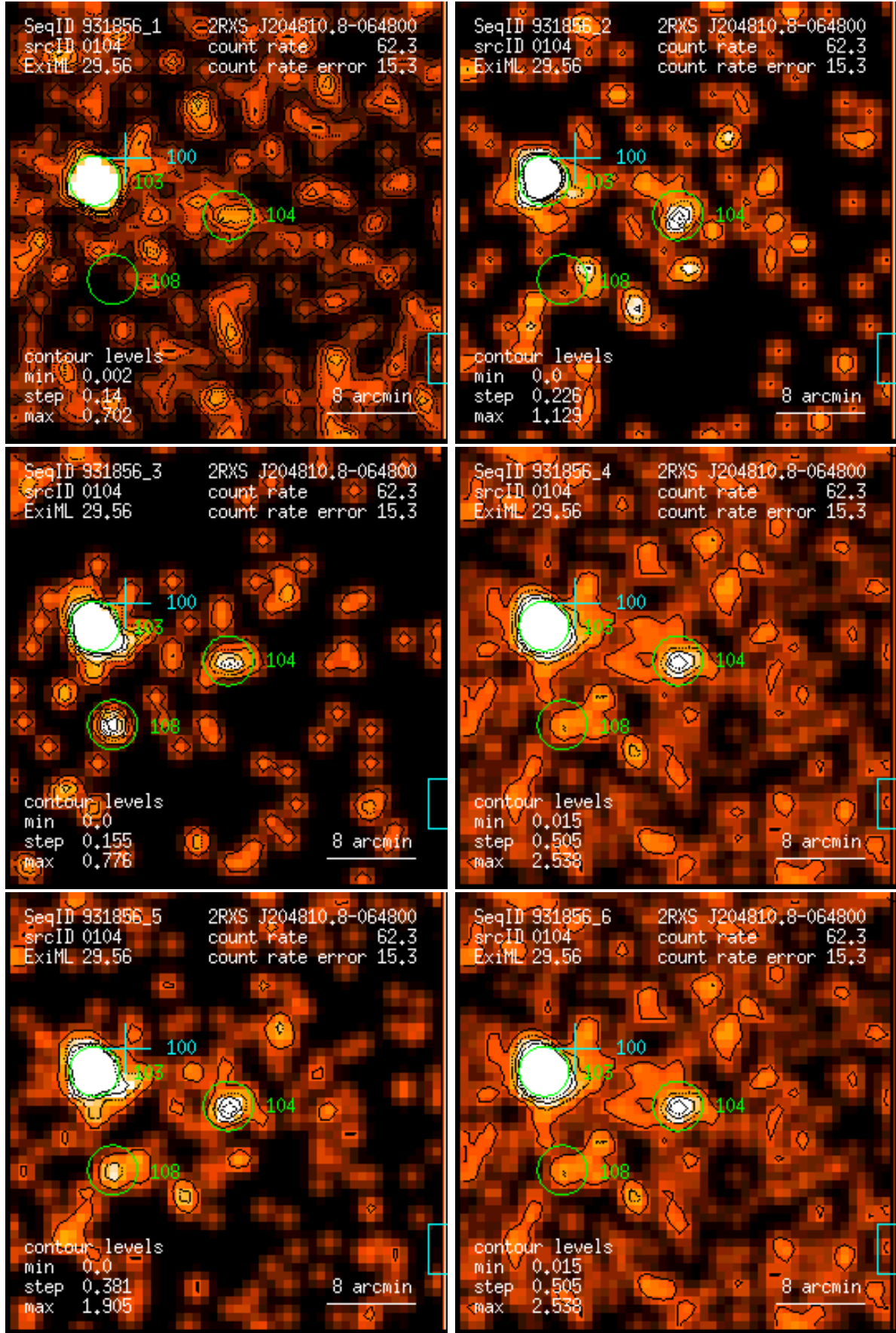
Figure 104: RASS 931856: detection 0104: band rate images, Gaussian filter: (1) PSPC channels 11 – 41, (2) 52 – 90, (3) 91 – 201, (4) 11 – 235, (5) 52 – 201, (6) 11 – 201. Broad band rates in counts/ks. Band rate contour levels in counts/ks/arcmin 2 .
