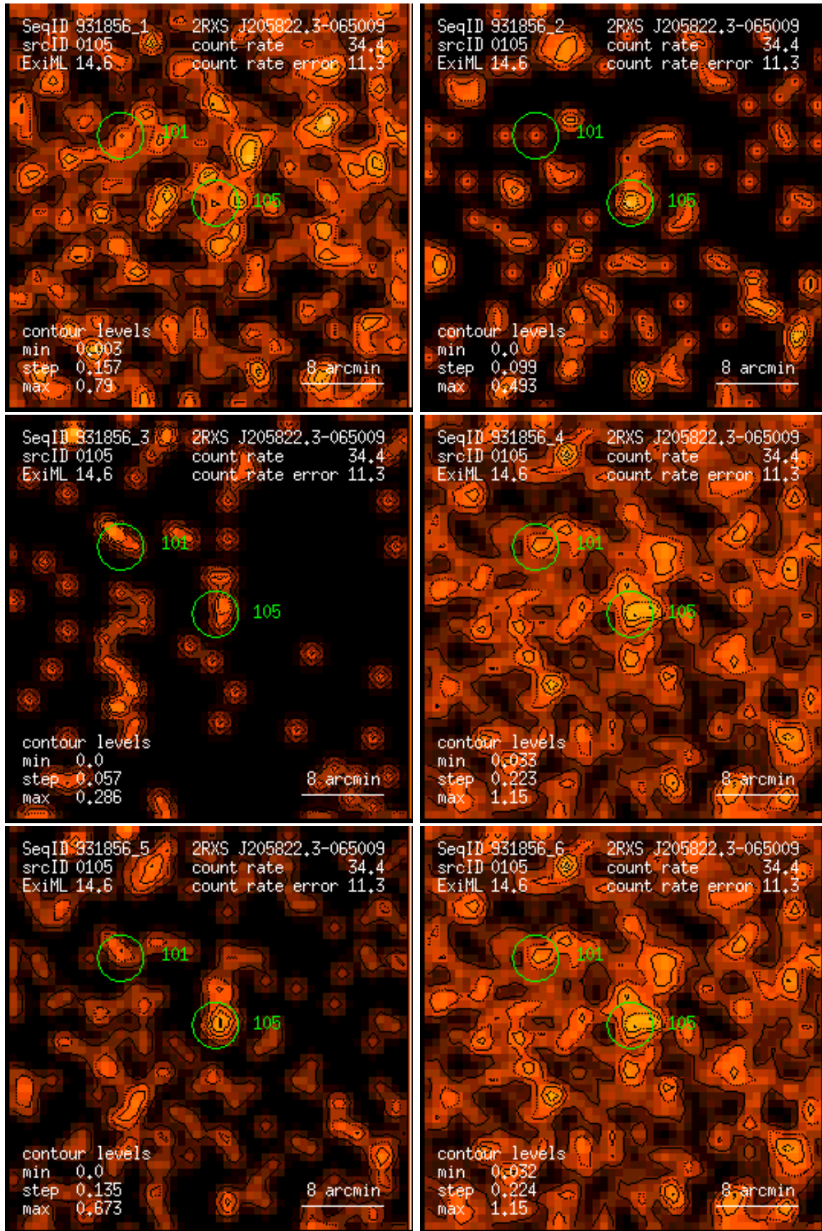
Figure 105: RASS 931856: detection 0105: band rate images, Gaussian filter: (1) PSPC channels 11 – 41, (2) 52 – 90, (3) 91 – 201, (4) 11 – 235, (5) 52 – 201, (6) 11 – 201. Broad band rates in counts/ks. Band rate contour levels in counts/ks/arcmin 2 .
