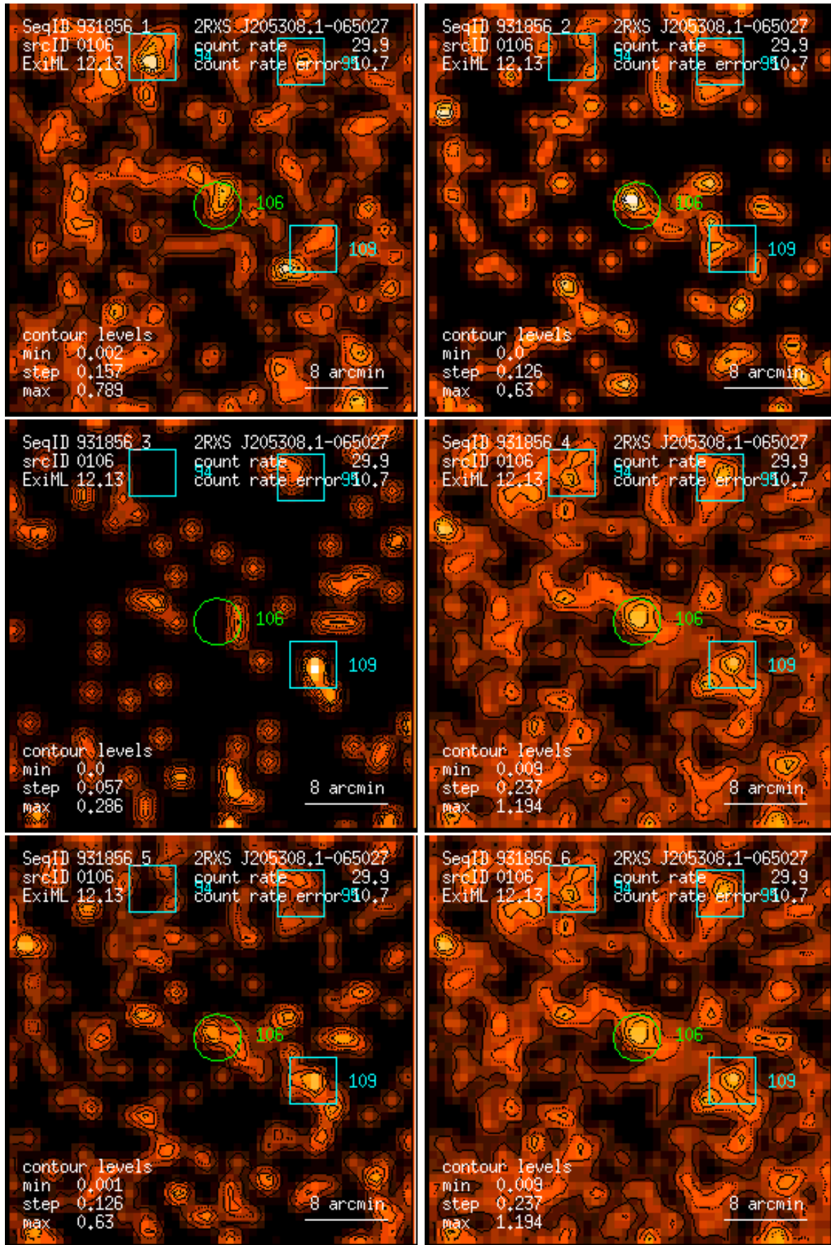
Figure 106: RASS 931856: detection 0106: band rate images, Gaussian filter: (1) PSPC channels 11 – 41, (2) 52 – 90, (3) 91 – 201, (4) 11 – 235, (5) 52 – 201, (6) 11 – 201. Broad band rates in counts/ks. Band rate contour levels in counts/ks/arcmin 2 .
