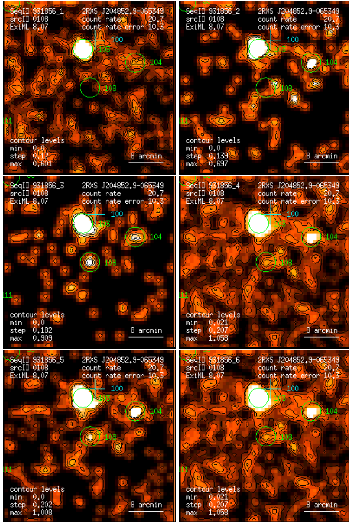
Figure 108: RASS 931856: detection 0108: band rate images, Gaussian filter: (1) PSPC channels 11 – 41, (2) 52 – 90, (3) 91 – 201, (4) 11 – 235, (5) 52 – 201, (6) 11 – 201. Broad band rates in counts/ks. Band rate contour levels in counts/ks/arcmin 2 .
