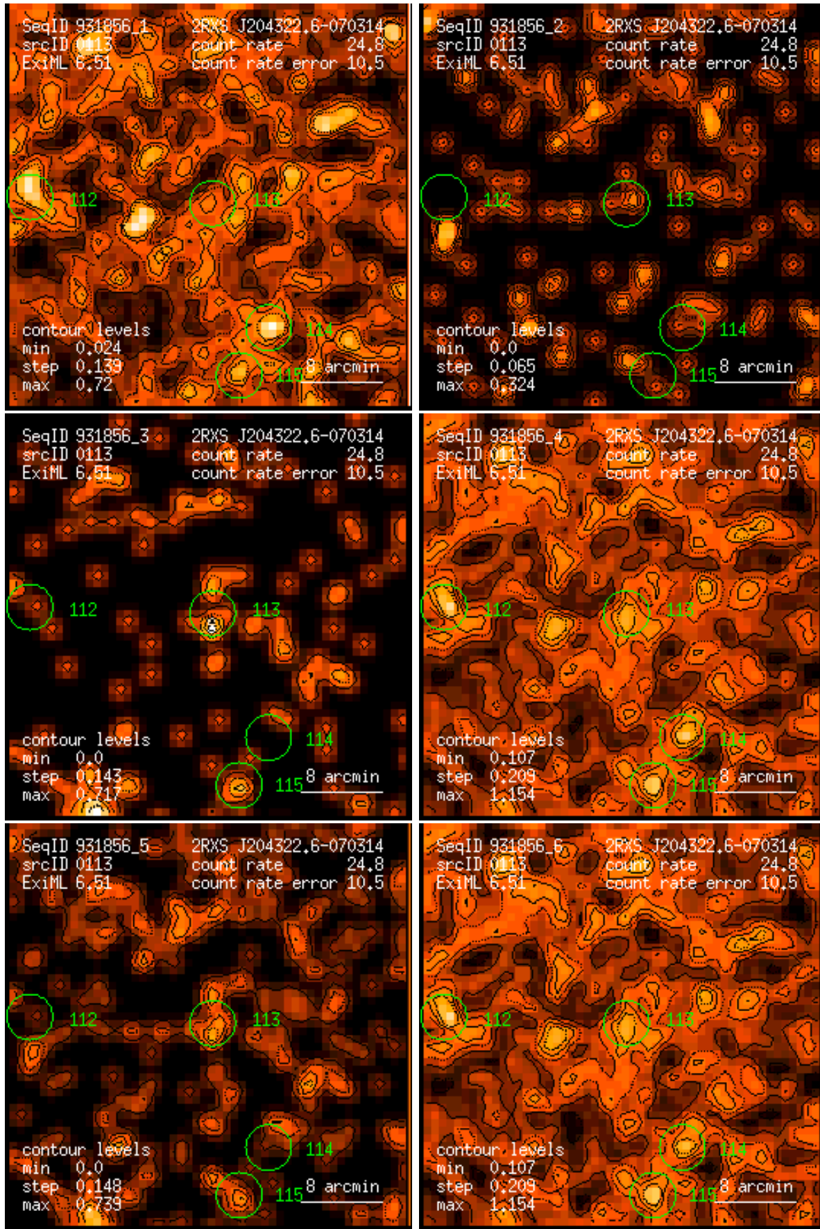
Figure 113: RASS 931856: detection 0113: band rate images, Gaussian filter: (1) PSPC channels 11 – 41, (2) 52 – 90, (3) 91 – 201, (4) 11 – 235, (5) 52 – 201, (6) 11 – 201. Broad band rates in counts/ks. Band rate contour levels in counts/ks/arcmin 2 .
