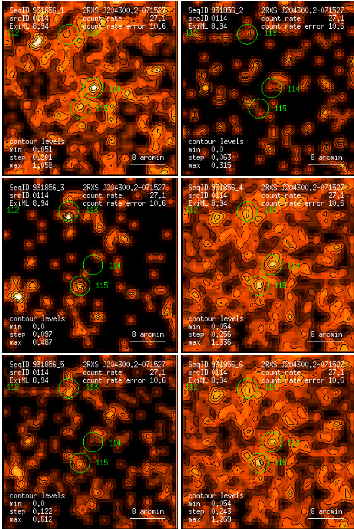
Figure 114: RASS 931856: detection 0114: band rate images, Gaussian filter: (1) PSPC channels 11 – 41, (2) 52 – 90, (3) 91 – 201, (4) 11 – 235, (5) 52 – 201, (6) 11 – 201. Broad band rates in counts/ks. Band rate contour levels in counts/ks/arcmin 2 .
