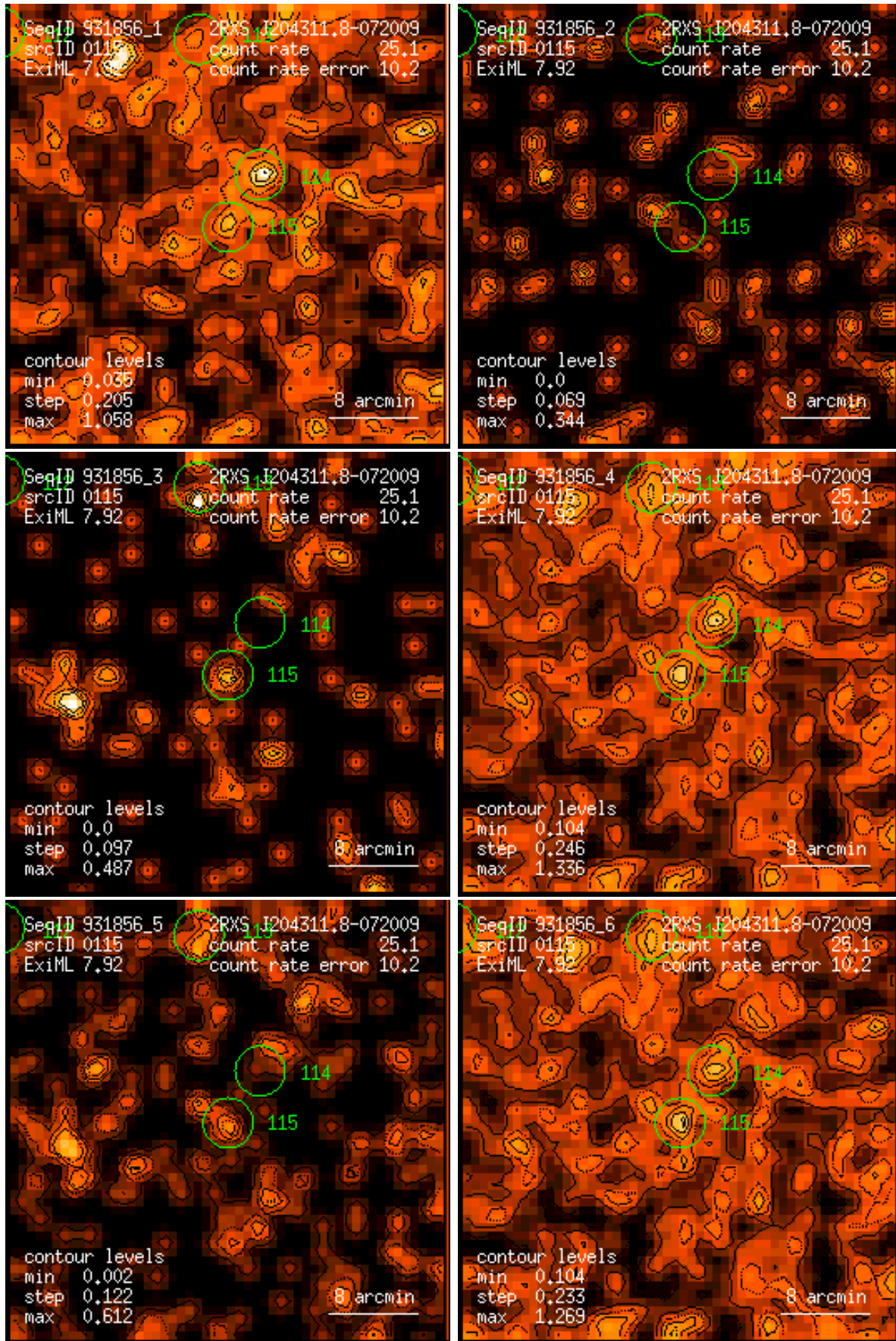
Figure 115: RASS 931856: detection 0115: band rate images, Gaussian filter: (1) PSPC channels 11 – 41, (2) 52 – 90, (3) 91 – 201, (4) 11 – 235, (5) 52 – 201, (6) 11 – 201. Broad band rates in counts/ks. Band rate contour levels in counts/ks/arcmin 2 .
