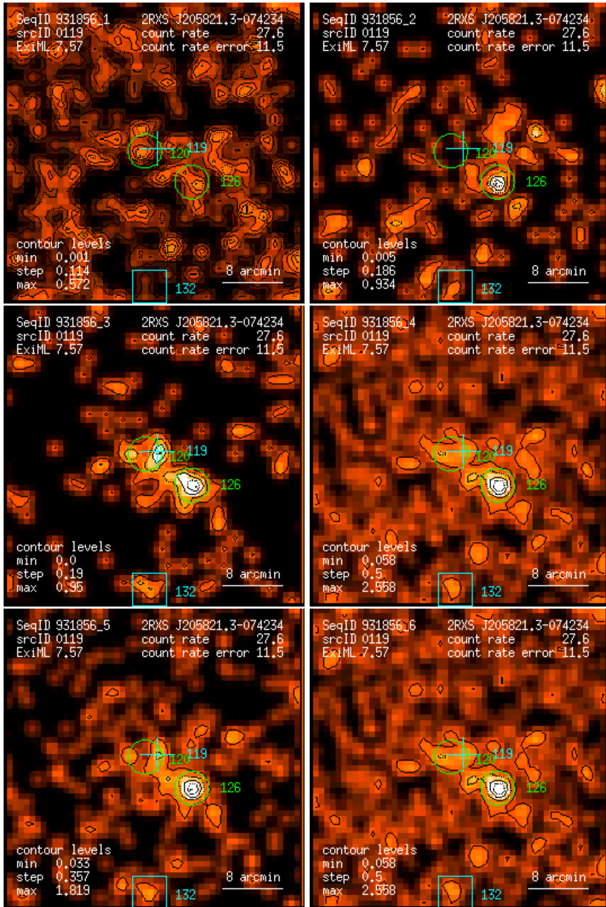
Figure 119: RASS 931856: detection 0119: band rate images, Gaussian filter: (1) PSPC channels 11 – 41, (2) 52 – 90, (3) 91 – 201, (4) 11 – 235, (5) 52 – 201, (6) 11 – 201. Broad band rates in counts/ks. Band rate contour levels in counts/ks/arcmin 2 .
