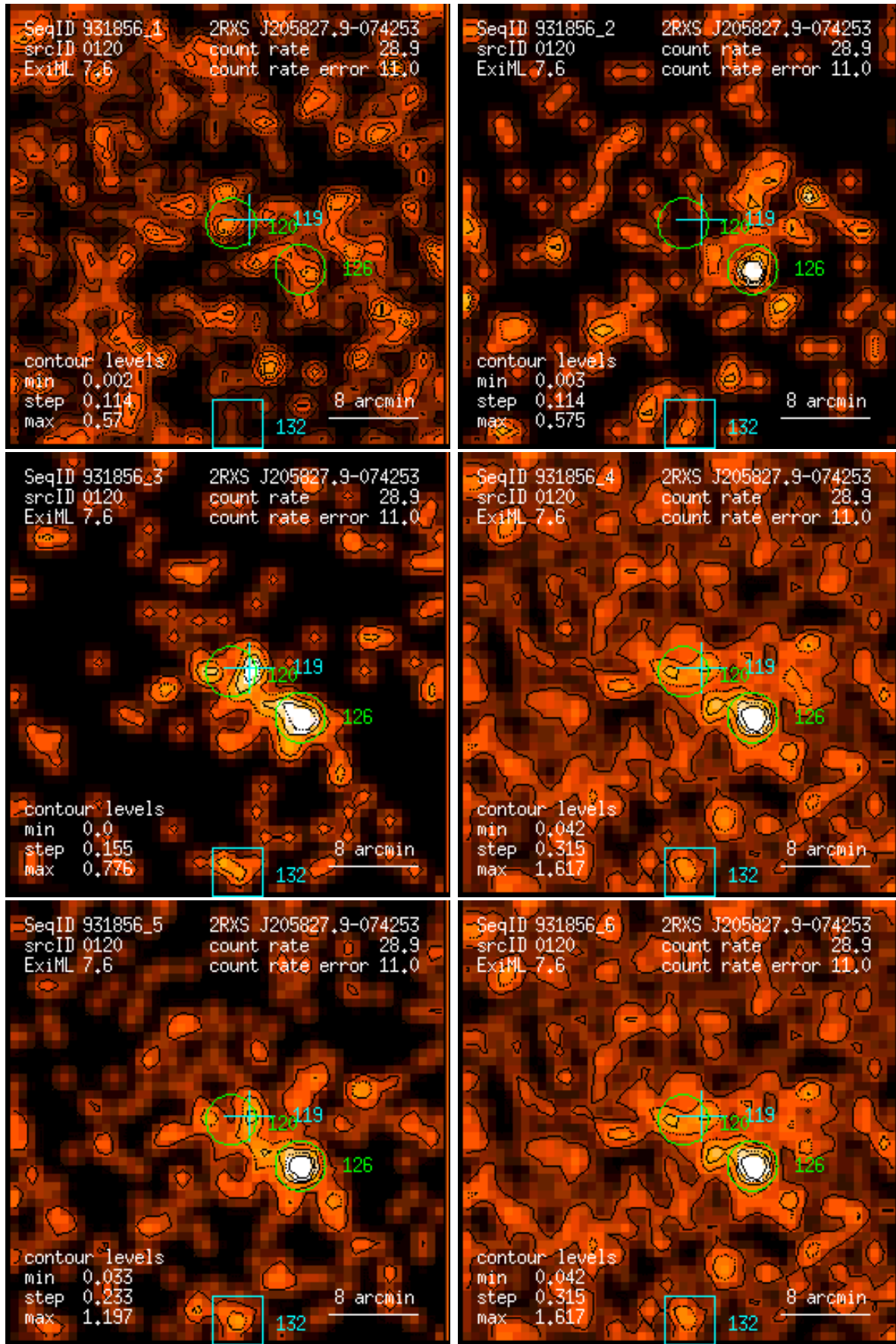
Figure 120: RASS 931856: detection 0120: band rate images, Gaussian filter: (1) PSPC channels 11 – 41, (2) 52 – 90, (3) 91 – 201, (4) 11 – 235, (5) 52 – 201, (6) 11 – 201. Broad band rates in counts/ks. Band rate contour levels in counts/ks/arcmin 2 .
