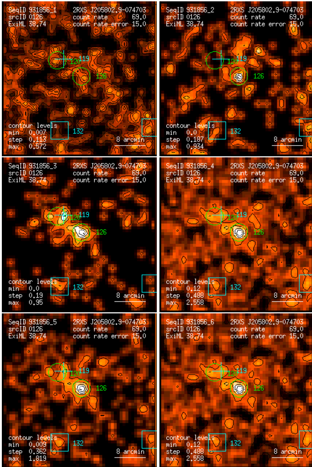
Figure 126: RASS 931856: detection 0126: band rate images, Gaussian filter: (1) PSPC channels 11 – 41, (2) 52 – 90, (3) 91 – 201, (4) 11 – 235, (5) 52 – 201, (6) 11 – 201. Broad band rates in counts/ks. Band rate contour levels in counts/ks/arcmin 2 .
