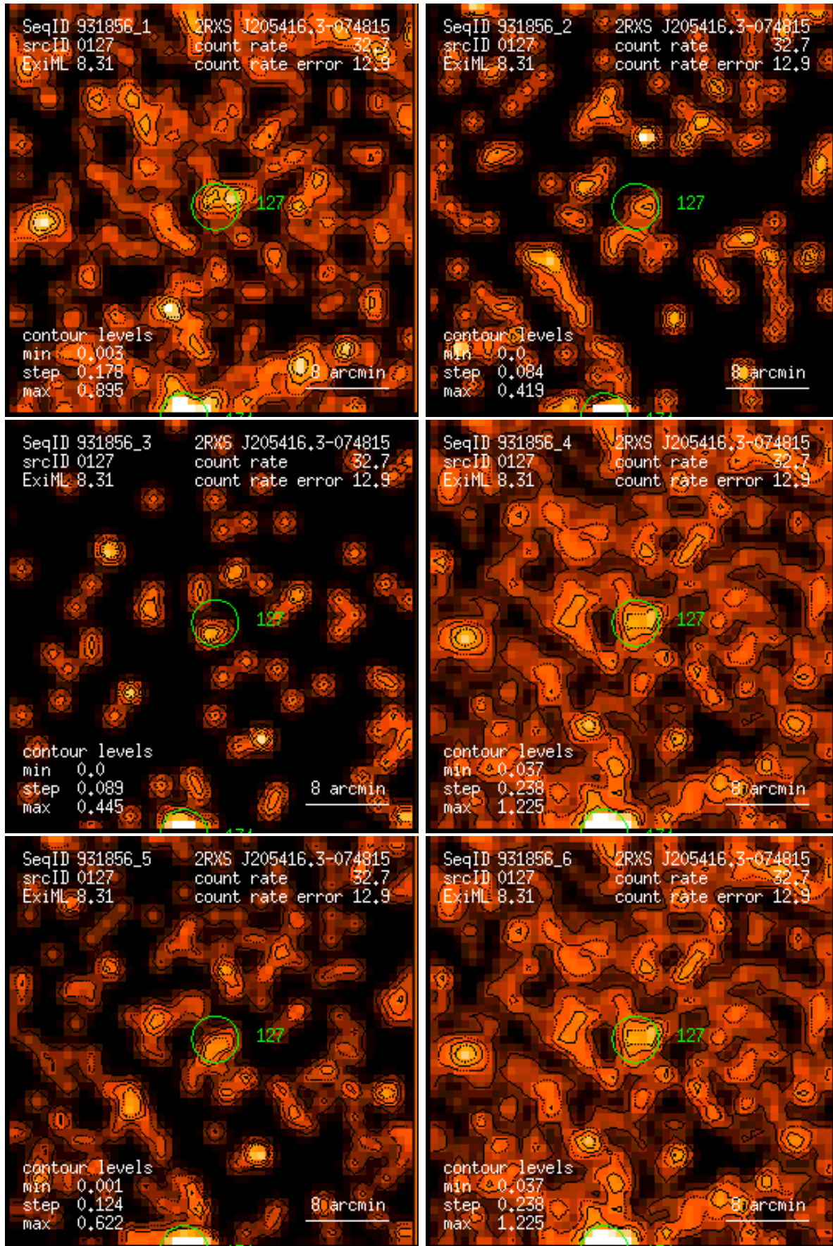
Figure 127: RASS 931856: detection 0127: band rate images, Gaussian filter: (1) PSPC channels 11 – 41, (2) 52 – 90, (3) 91 – 201, (4) 11 – 235, (5) 52 – 201, (6) 11 – 201. Broad band rates in counts/ks. Band rate contour levels in counts/ks/arcmin 2 .
