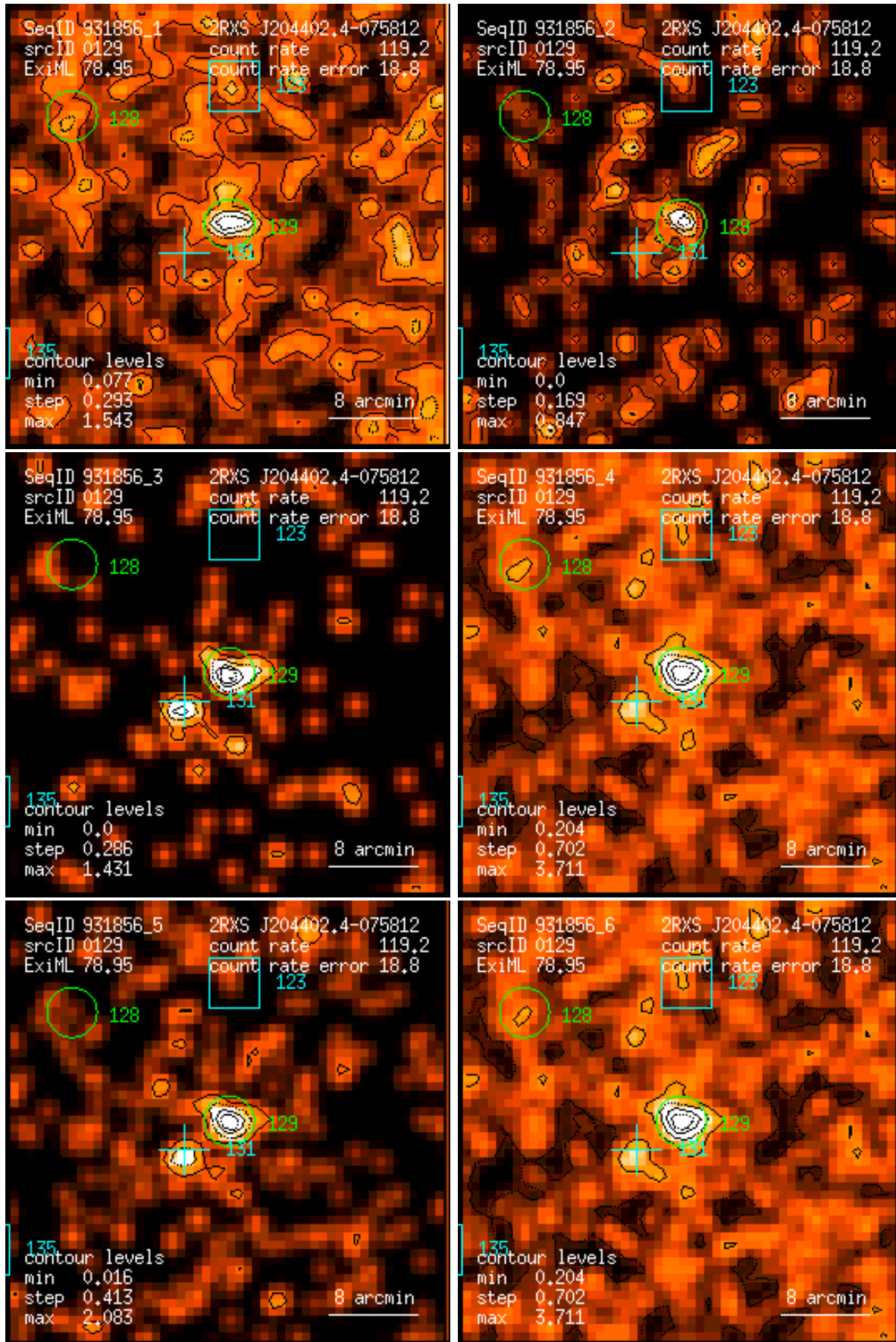
Figure 129: RASS 931856: detection 0129: band rate images, Gaussian filter: (1) PSPC channels 11 – 41, (2) 52 – 90, (3) 91 – 201, (4) 11 – 235, (5) 52 – 201, (6) 11 – 201. Broad band rates in counts/ks. Band rate contour levels in counts/ks/arcmin 2 .
