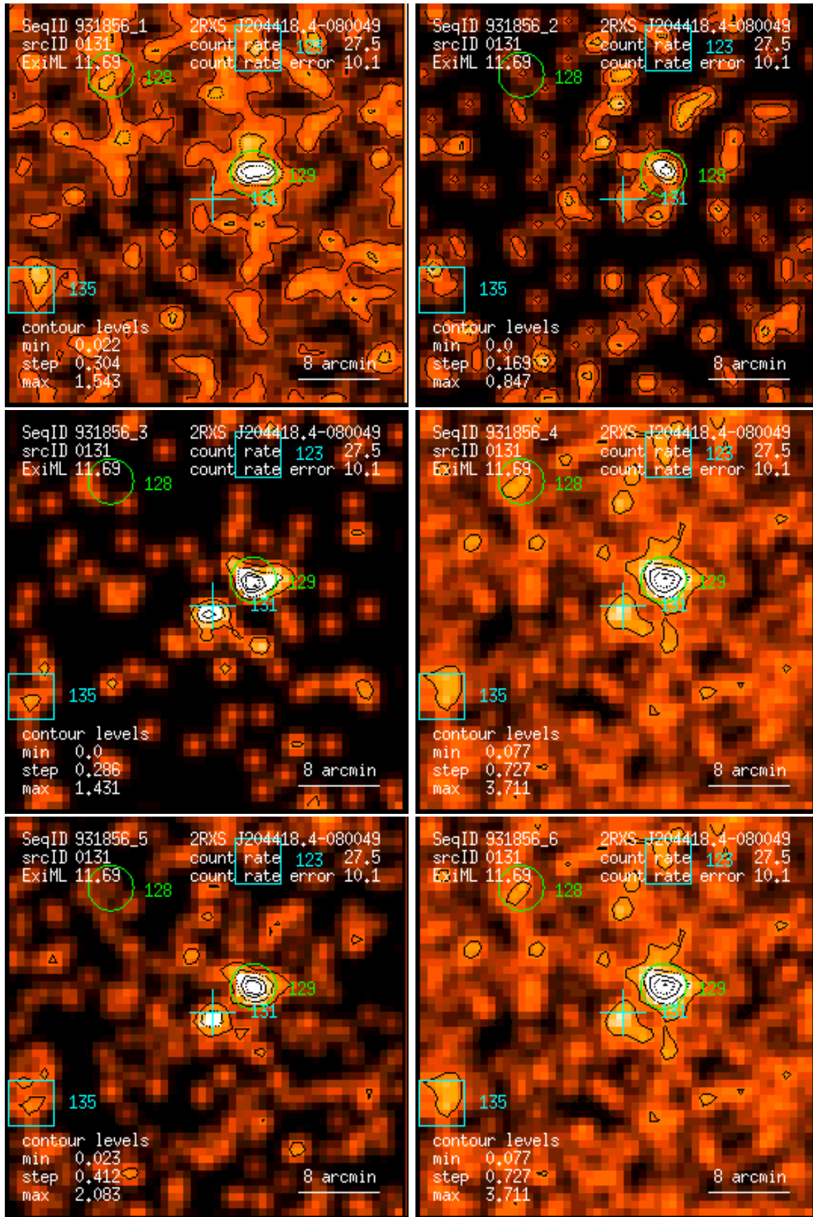
Figure 131: RASS 931856: detection 0131: band rate images, Gaussian filter: (1) PSPC channels 11 – 41, (2) 52 – 90, (3) 91 – 201, (4) 11 – 235, (5) 52 – 201, (6) 11 – 201. Broad band rates in counts/ks. Band rate contour levels in counts/ks/arcmin 2 .
