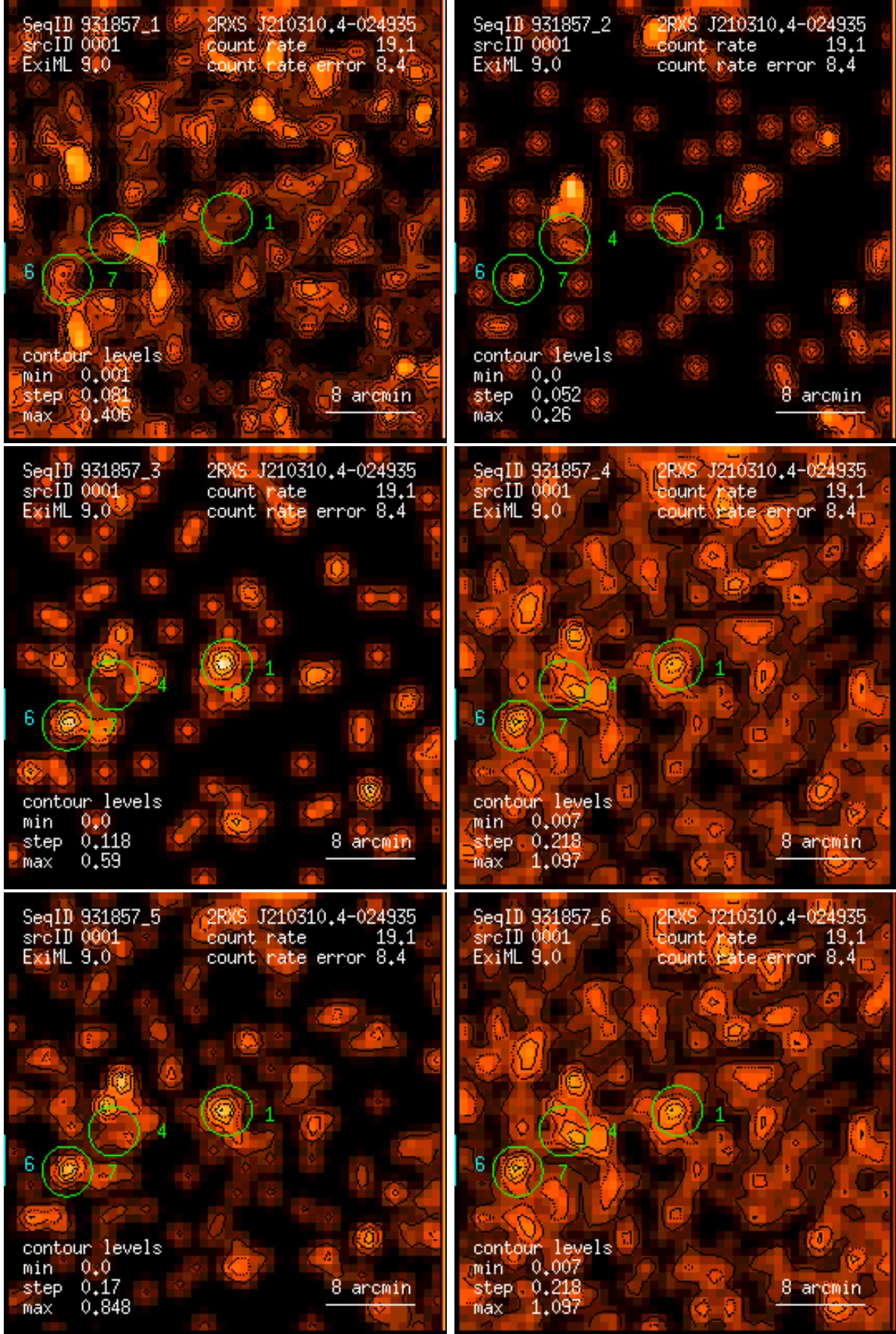
Figure 1: RASS 931857: detection 0001: band rate images, Gaussian filter: (1) PSPC channels 11 – 41, (2) 52 – 90, (3) 91 – 201, (4) 11 – 235, (5) 52 – 201, (6) 11 – 201. Broad band rates in counts/ks. Band rate contour levels in counts/ks/arcmin 2 .
