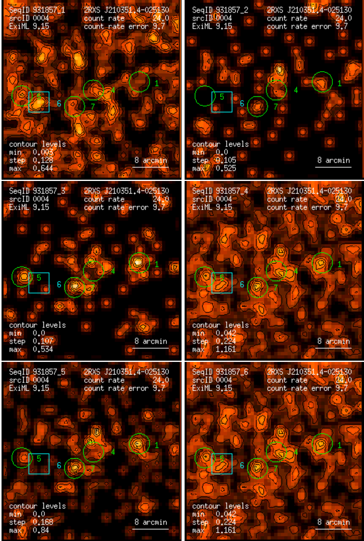
Figure 4: RASS 931857: detection 0004: band rate images, Gaussian filter: (1) PSPC channels 11 – 41, (2) 52 – 90, (3) 91 – 201, (4) 11 – 235, (5) 52 – 201, (6) 11 – 201. Broad band rates in counts/ks. Band rate contour levels in counts/ks/arcmin 2 .
