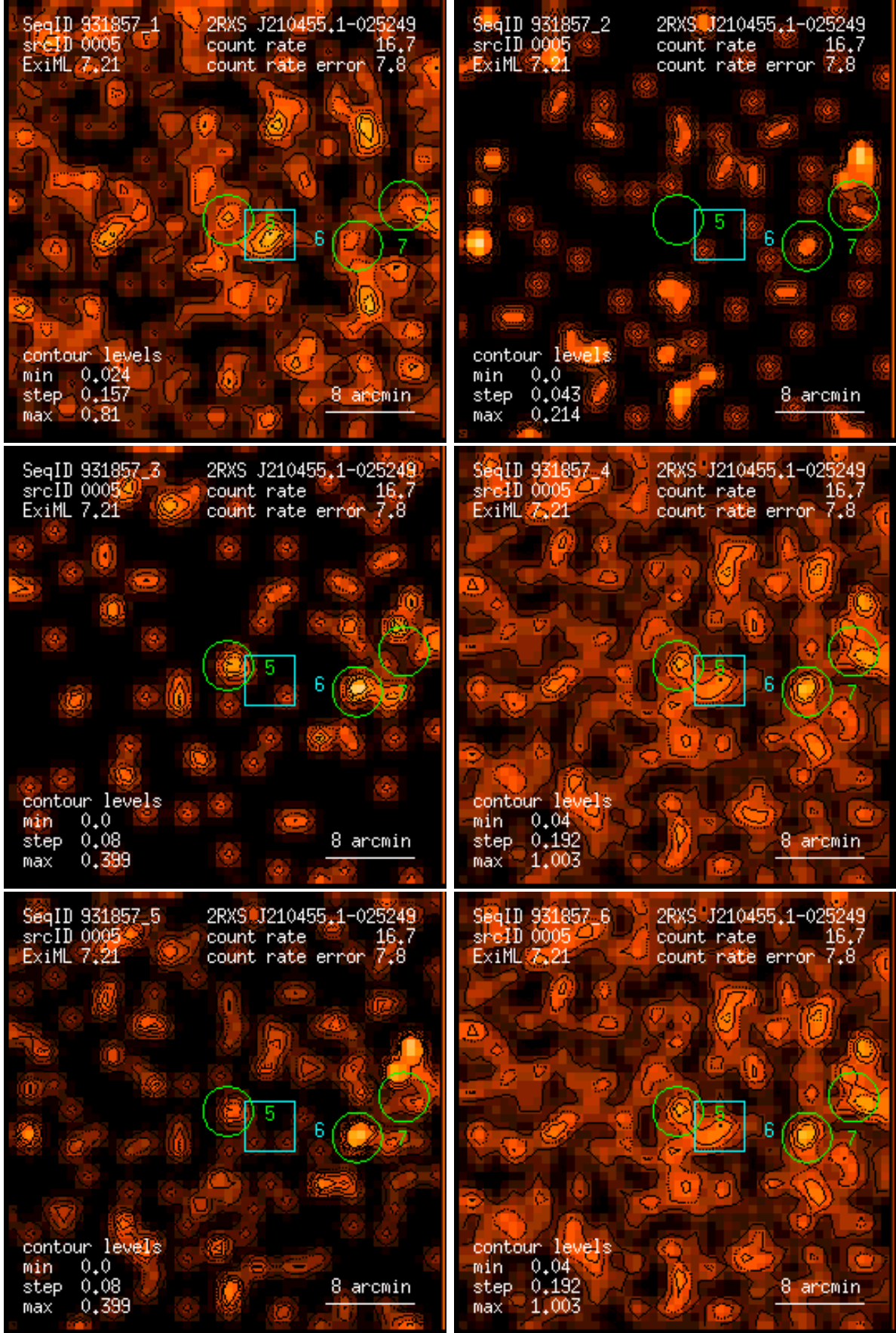
Figure 5: RASS 931857: detection 0005: band rate images, Gaussian filter: (1) PSPC channels 11 – 41, (2) 52 – 90, (3) 91 – 201, (4) 11 – 235, (5) 52 – 201, (6) 11 – 201. Broad band rates in counts/ks. Band rate contour levels in counts/ks/arcmin 2 .
