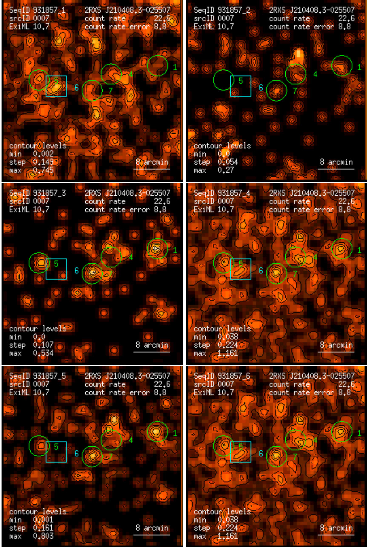
Figure 7: RASS 931857: detection 0007: band rate images, Gaussian filter: (1) PSPC channels 11 – 41, (2) 52 – 90, (3) 91 – 201, (4) 11 – 235, (5) 52 – 201, (6) 11 – 201. Broad band rates in counts/ks. Band rate contour levels in counts/ks/arcmin 2 .
