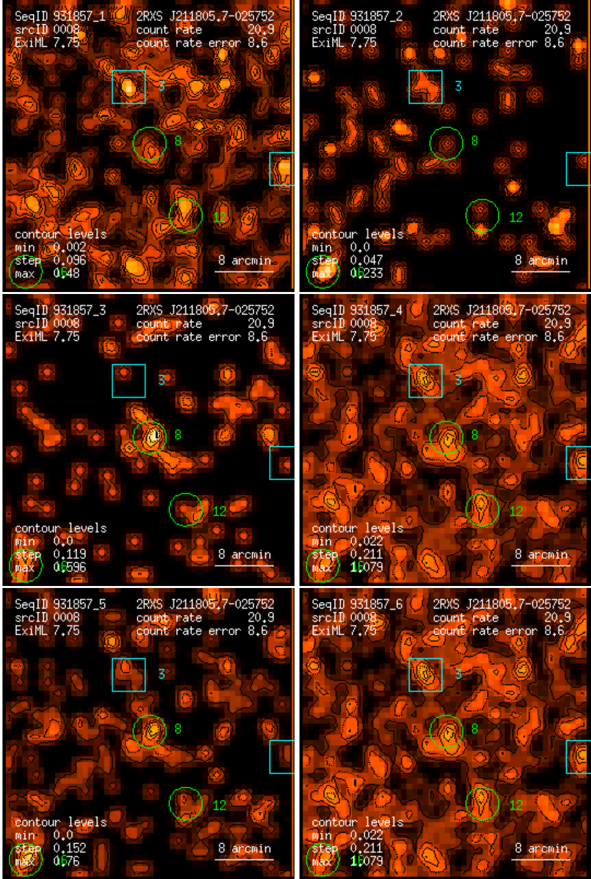
Figure 8: RASS 931857: detection 0008: band rate images, Gaussian filter: (1) PSPC channels 11 – 41, (2) 52 – 90, (3) 91 – 201, (4) 11 – 235, (5) 52 – 201, (6) 11 – 201. Broad band rates in counts/ks. Band rate contour levels in counts/ks/arcmin 2 .
