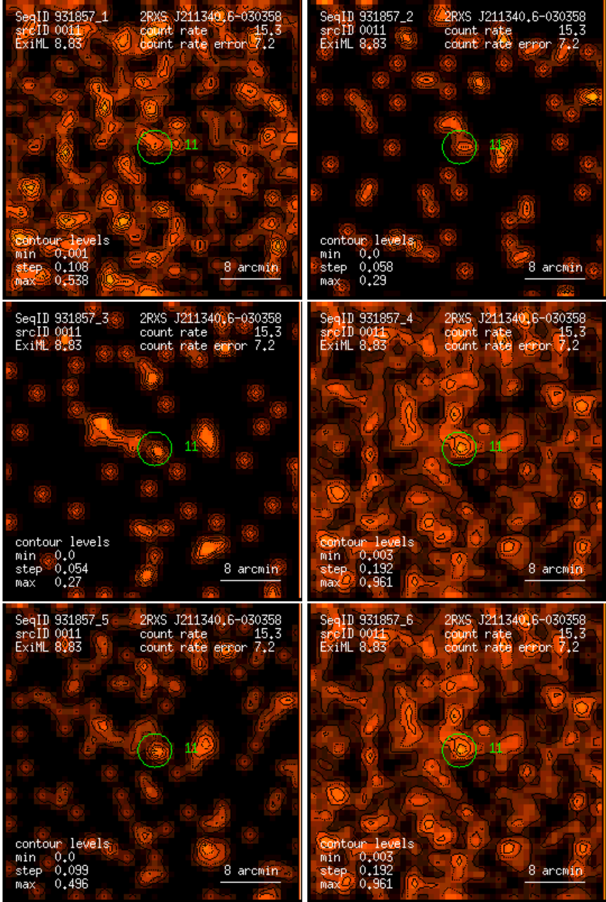
Figure 11: RASS 931857: detection 0011: band rate images, Gaussian filter: (1) PSPC channels 11 – 41, (2) 52 – 90, (3) 91 – 201, (4) 11 – 235, (5) 52 – 201, (6) 11 – 201. Broad band rates in counts/ks. Band rate contour levels in counts/ks/arcmin 2 .
