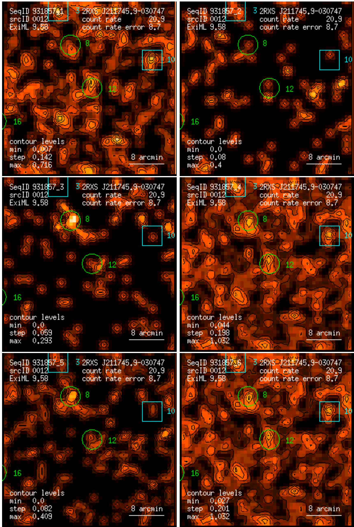
Figure 12: RASS 931857: detection 0012: band rate images, Gaussian filter: (1) PSPC channels 11 – 41, (2) 52 – 90, (3) 91 – 201, (4) 11 – 235, (5) 52 – 201, (6) 11 – 201. Broad band rates in counts/ks. Band rate contour levels in counts/ks/arcmin 2 .
