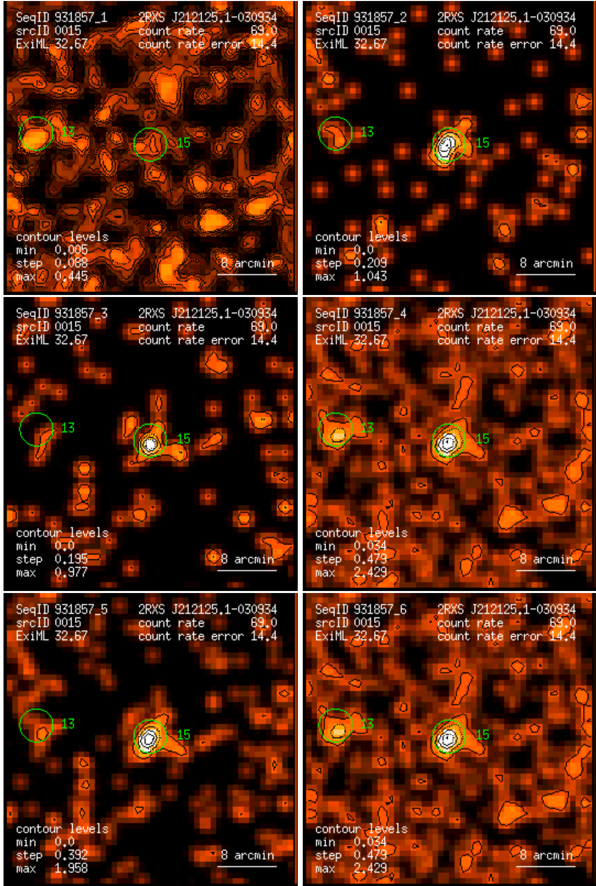
Figure 15: RASS 931857: detection 0015: band rate images, Gaussian filter: (1) PSPC channels 11 – 41, (2) 52 – 90, (3) 91 – 201, (4) 11 – 235, (5) 52 – 201, (6) 11 – 201. Broad band rates in counts/ks. Band rate contour levels in counts/ks/arcmin 2 .
