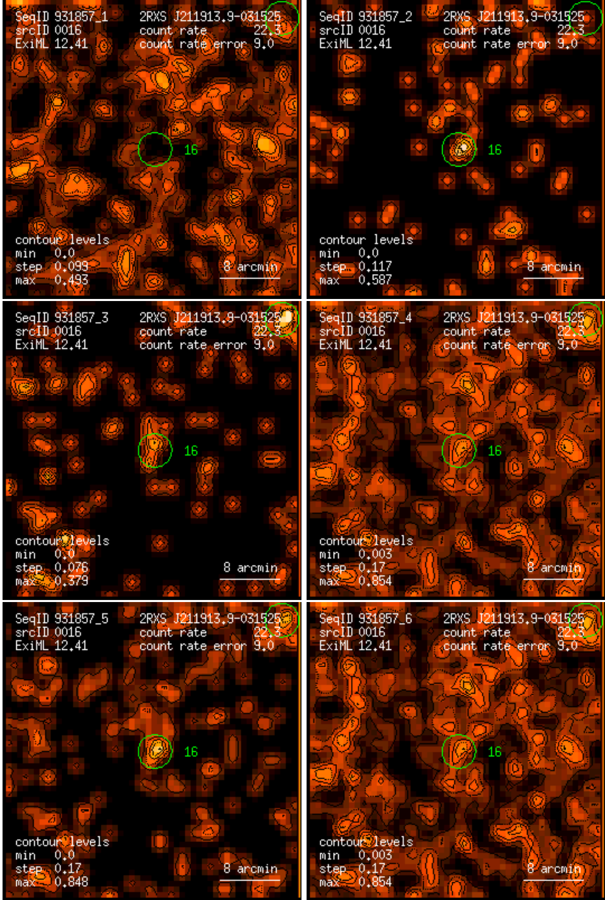
Figure 16: RASS 931857: detection 0016: band rate images, Gaussian filter: (1) PSPC channels 11 – 41, (2) 52 – 90, (3) 91 – 201, (4) 11 – 235, (5) 52 – 201, (6) 11 – 201. Broad band rates in counts/ks. Band rate contour levels in counts/ks/arcmin 2 .
