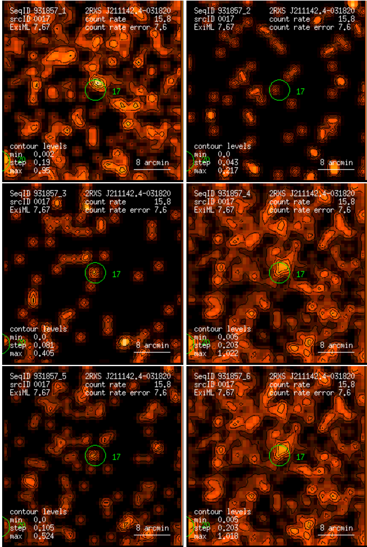
Figure 17: RASS 931857: detection 0017: band rate images, Gaussian filter: (1) PSPC channels 11 – 41, (2) 52 – 90, (3) 91 – 201, (4) 11 – 235, (5) 52 – 201, (6) 11 – 201. Broad band rates in counts/ks. Band rate contour levels in counts/ks/arcmin 2 .
