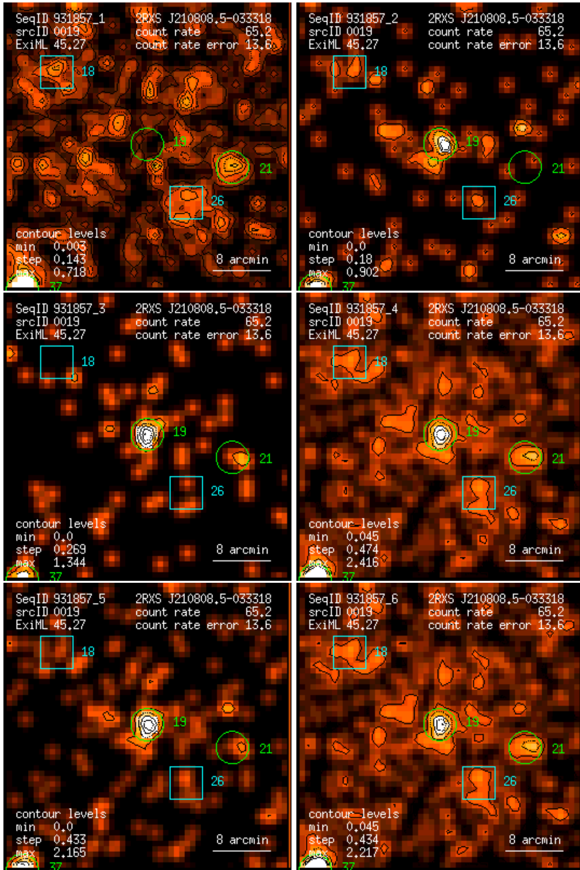
Figure 19: RASS 931857: detection 0019: band rate images, Gaussian filter: (1) PSPC channels 11 – 41, (2) 52 – 90, (3) 91 – 201, (4) 11 – 235, (5) 52 – 201, (6) 11 – 201. Broad band rates in counts/ks. Band rate contour levels in counts/ks/arcmin 2 .
