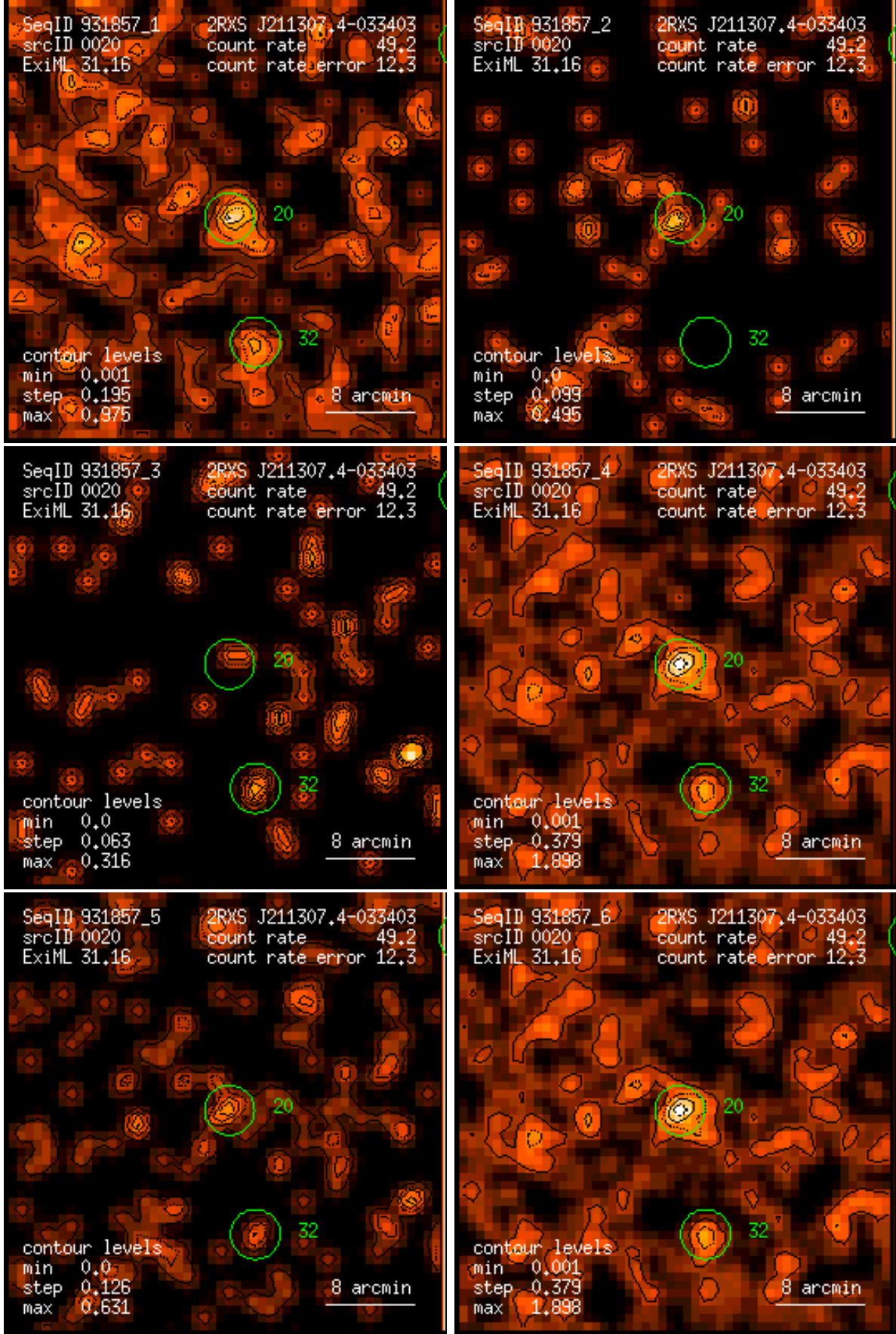
Figure 20: RASS 931857: detection 0020: band rate images, Gaussian filter: (1) PSPC channels 11 – 41, (2) 52 – 90, (3) 91 – 201, (4) 11 – 235, (5) 52 – 201, (6) 11 – 201. Broad band rates in counts/ks. Band rate contour levels in counts/ks/arcmin 2 .
