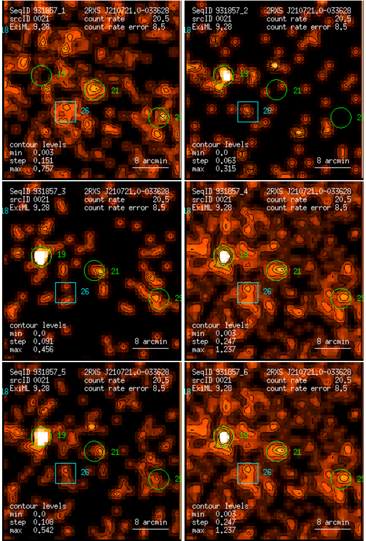
Figure 21: RASS 931857: detection 0021: band rate images, Gaussian filter: (1) PSPC channels 11 – 41, (2) 52 – 90, (3) 91 – 201, (4) 11 – 235, (5) 52 – 201, (6) 11 – 201. Broad band rates in counts/ks. Band rate contour levels in counts/ks/arcmin 2 .
